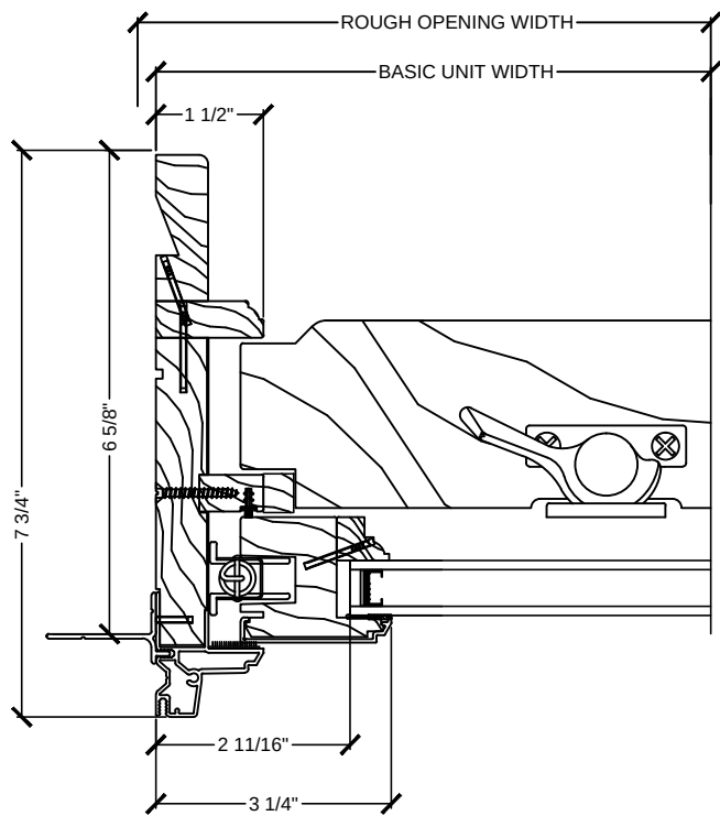
JAMB DETAIL MONUMENT CLAD DOUBLE HUNG WINDOW
