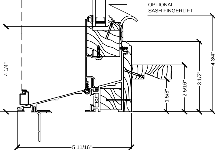
SILL DETAIL MONUMENT CLAD DOUBLE HUNG WINDOW
