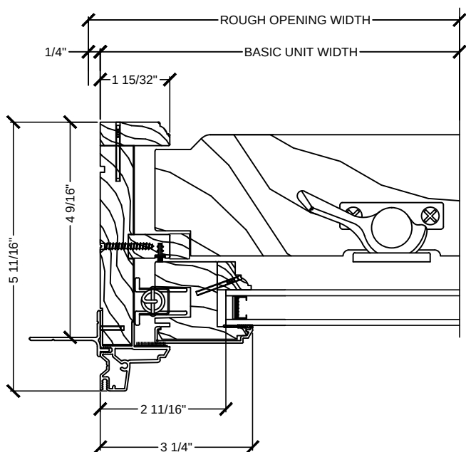
A 2 JAMB DETAIL MONUMENT CLAD DOUBLE HUNG WINDOW
