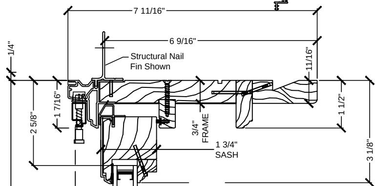
HEAD DETAIL MONUMENT CLAD DOUBLE HUNG WINDOW VINYL FOLDING NAIL FIN ALSO AVAILABLE
