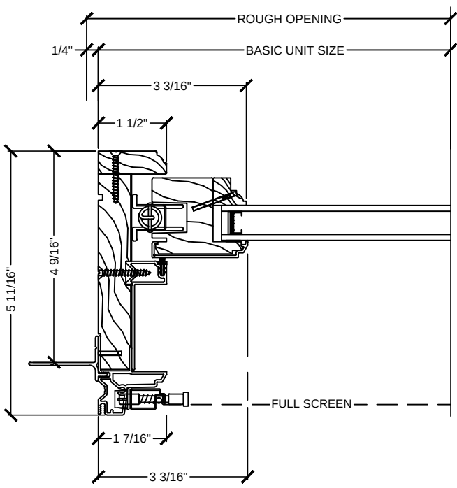
D 2 JAMB DETAIL MONUMENT CLAD DOUBLE HUNG WINDOW
