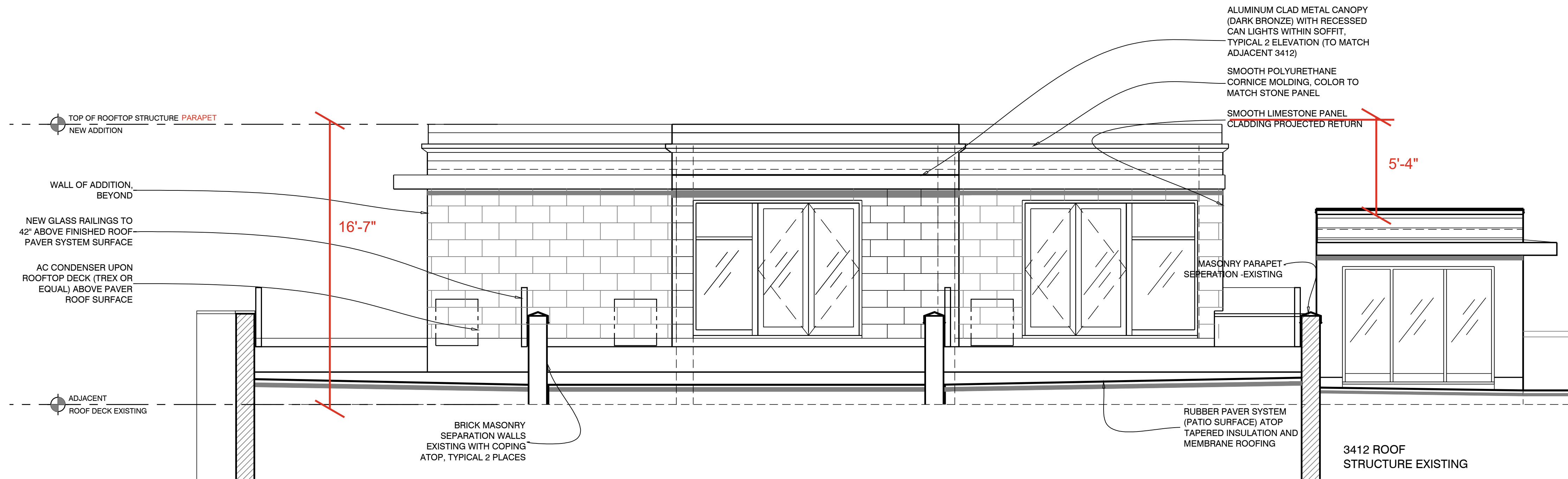
2 ROOFTOP JOHN R ELEVATION- WEST A2-3 SCALE: 1/4" = 1'-0"
