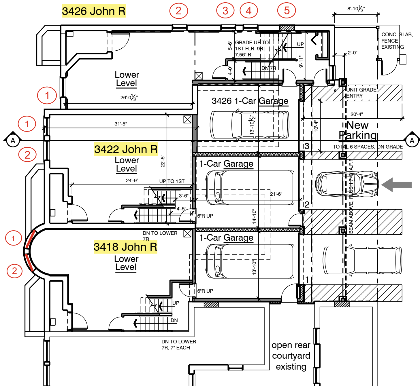
Lower Level Floor Plan - John R NEW PHASE
