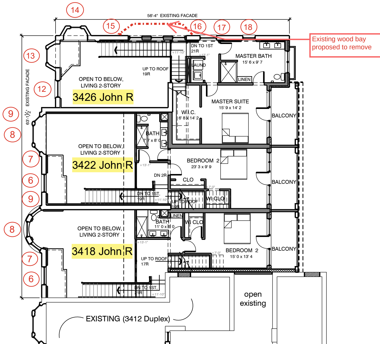
3rd Floor Plan - EXISTING WINDOW KEY NO SCALE
