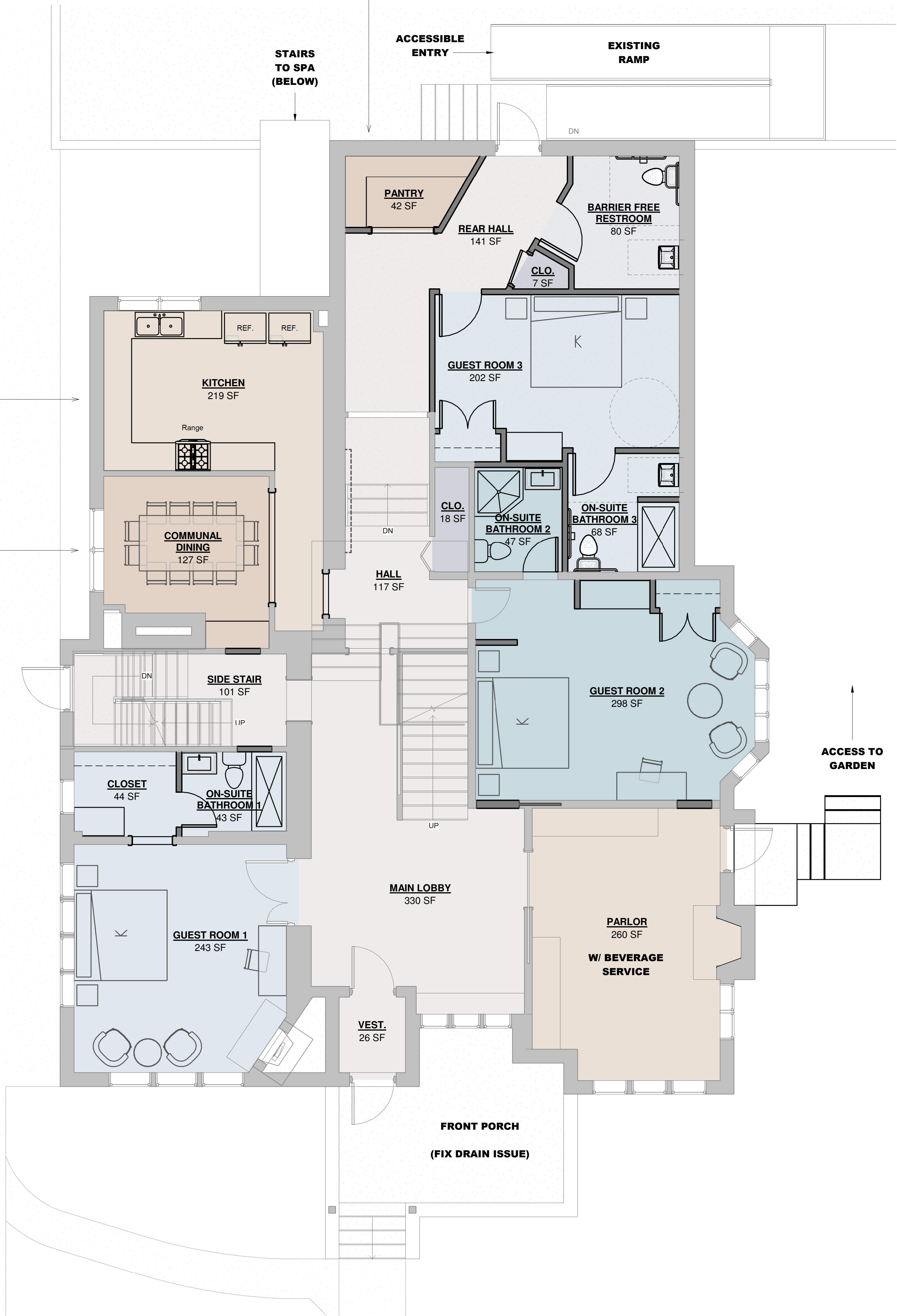
1 FIRST FLOOR - PROPOSED 1/4" = 1'-0"
