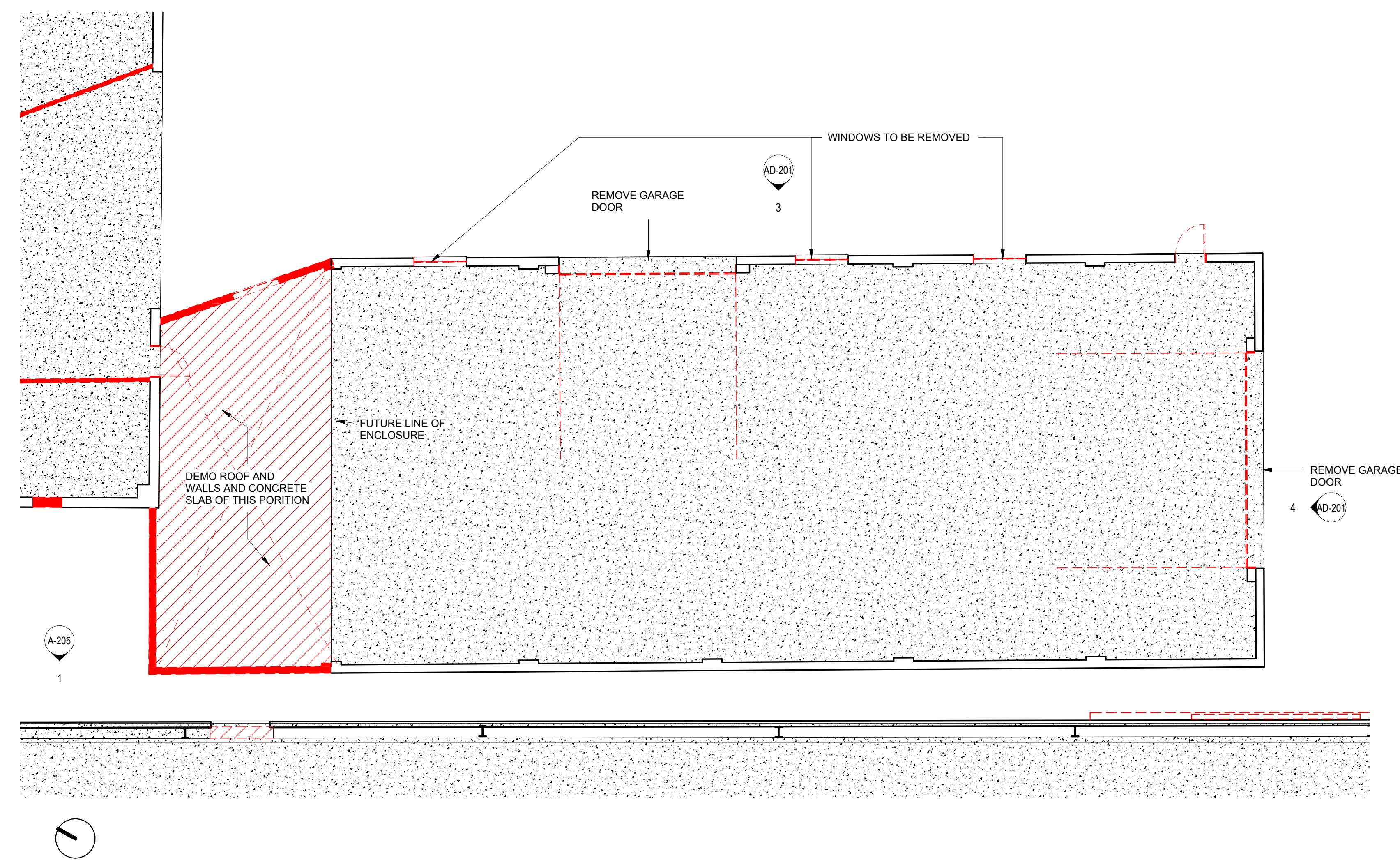
2 Workshop - Demolition Plan 1/8" = 1'-0"
