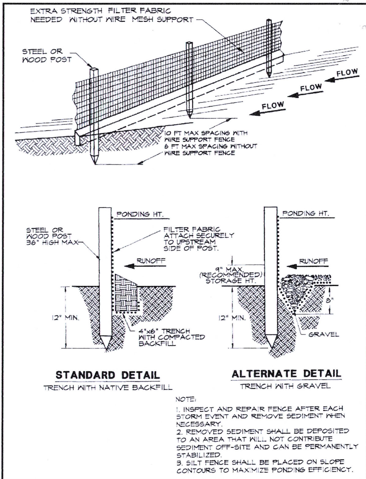
Figure 4.4a. Silt Fence
