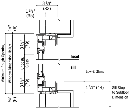
Vertical Section
