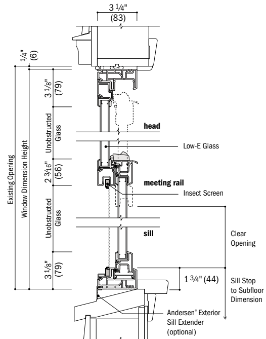
Vertical Section
