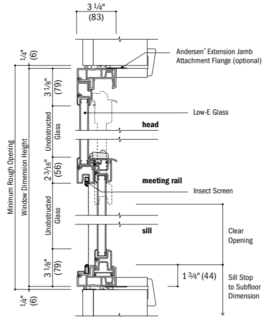
Vertical Section
