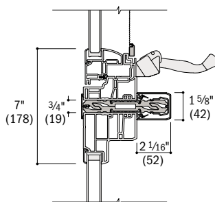
Awning Over Picture/Single Transom
