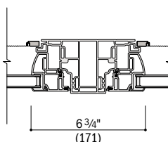
Horizontal Section Twin Casement
