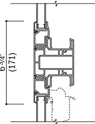
Vertical Section Transom Over Single-Hung
