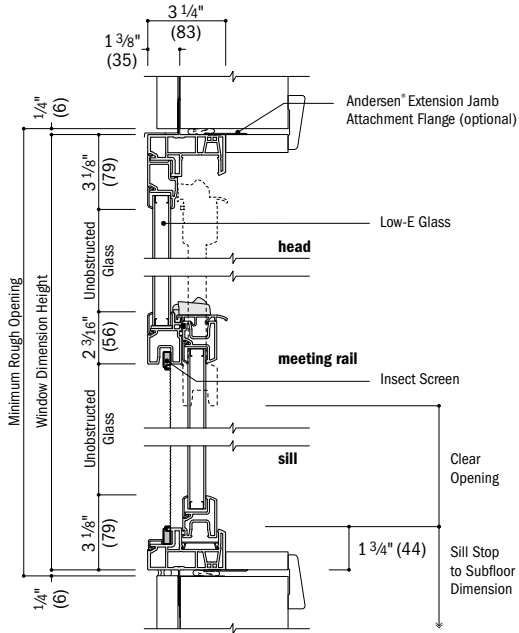
Vertical Section
