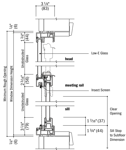
Vertical Section
