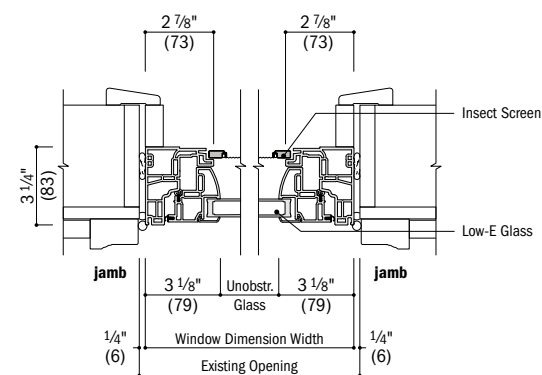
Horizontal Section Existing Window Opening
