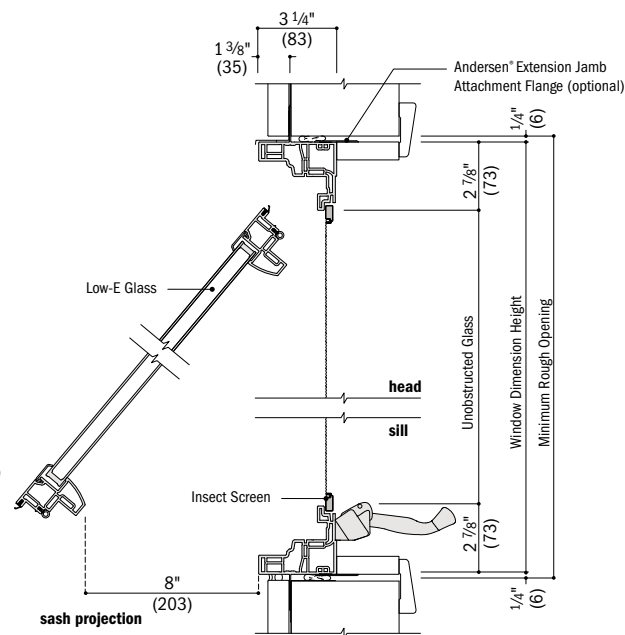
Vertical Section
