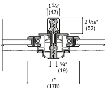
Single-Hung to Single-Hung
