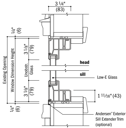
Vertical Section Existing Window Opening
