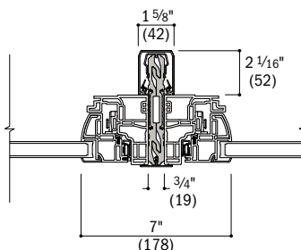
Awning to Awning
