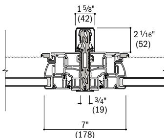
Casement to Casement (Hinge Jamb to Hinge Jamb)
