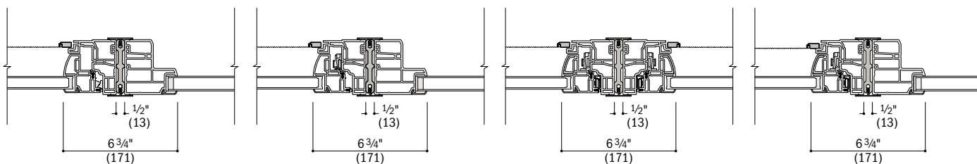
Casement to Picture/Single Transom (Casement Hinge Jamb)
