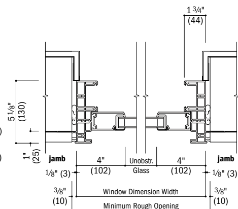
Horizontal Section Patio Door Sidelight/Transom – Stucco Exterior
