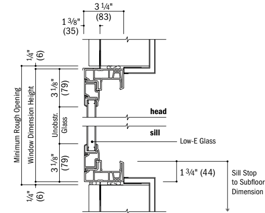
Vertical Section
