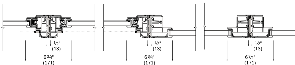
Single-Hung to Single-Hung
