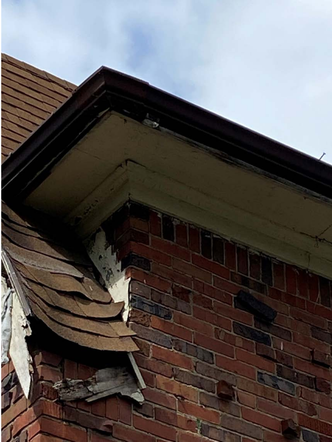
4 - Corner Gutter (Soth - East)
