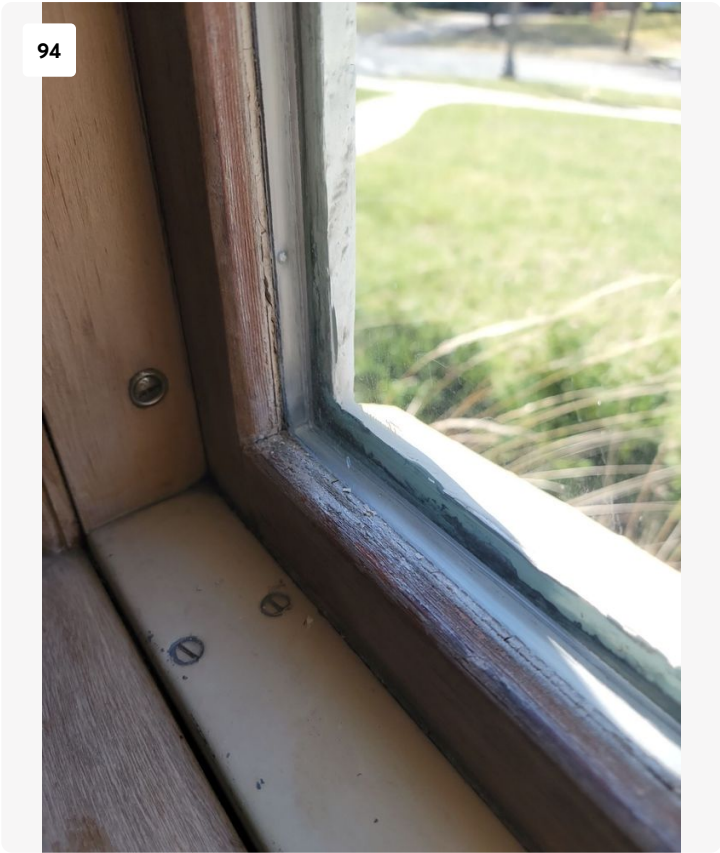
600-Mold, water damage, broken seals, decayed wood inside of glass, condensation inside of glass
