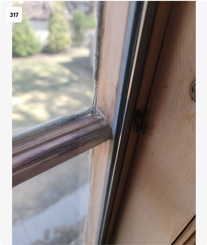
2600- water damage, mold, broken seals, hardware is non functioning, window does not open, condensation between glass, decayed wood between glass
