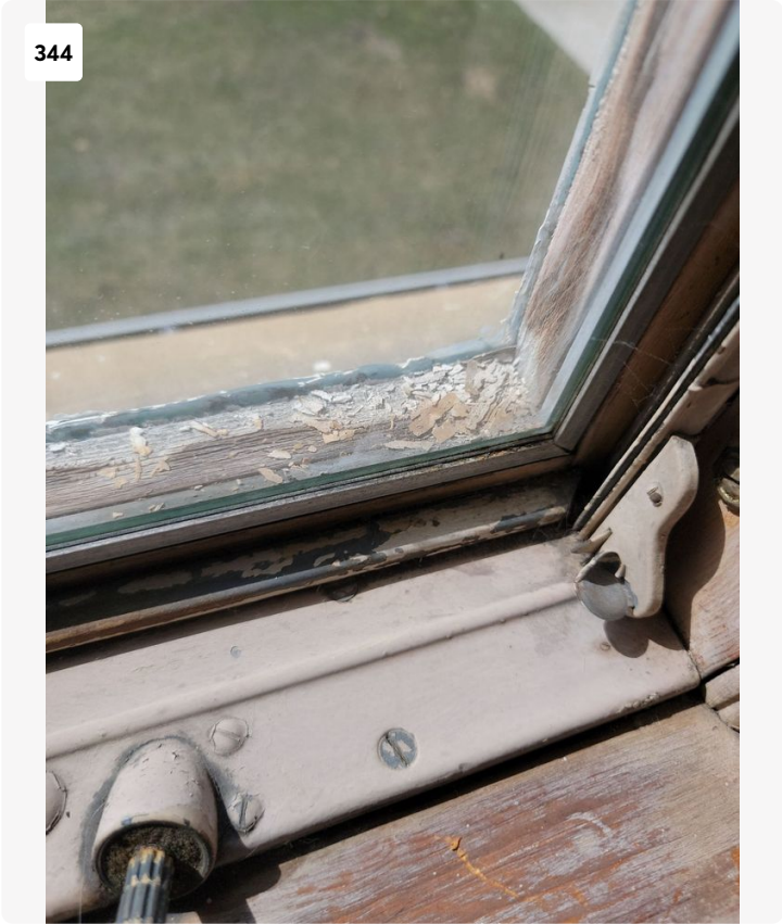
2800- water damage, mold, broken seals, hardware is non functioning, window does not open, condensation between glass, decayed wood between glass
