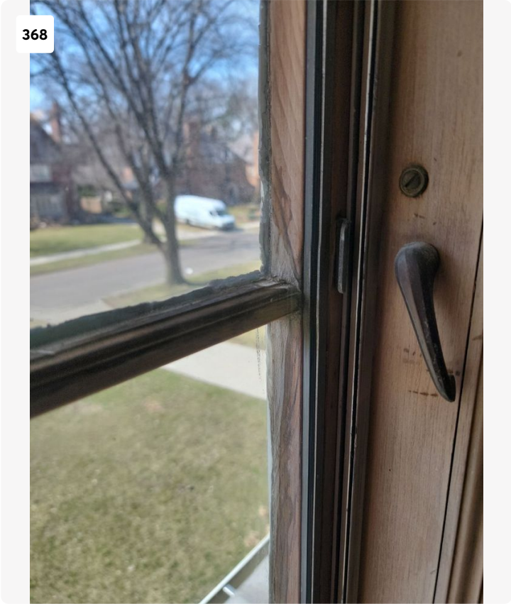
3200- water damage, mold, broken seals, hardware is non functioning, window does not open, condensation between glass, decayed wood between glass
