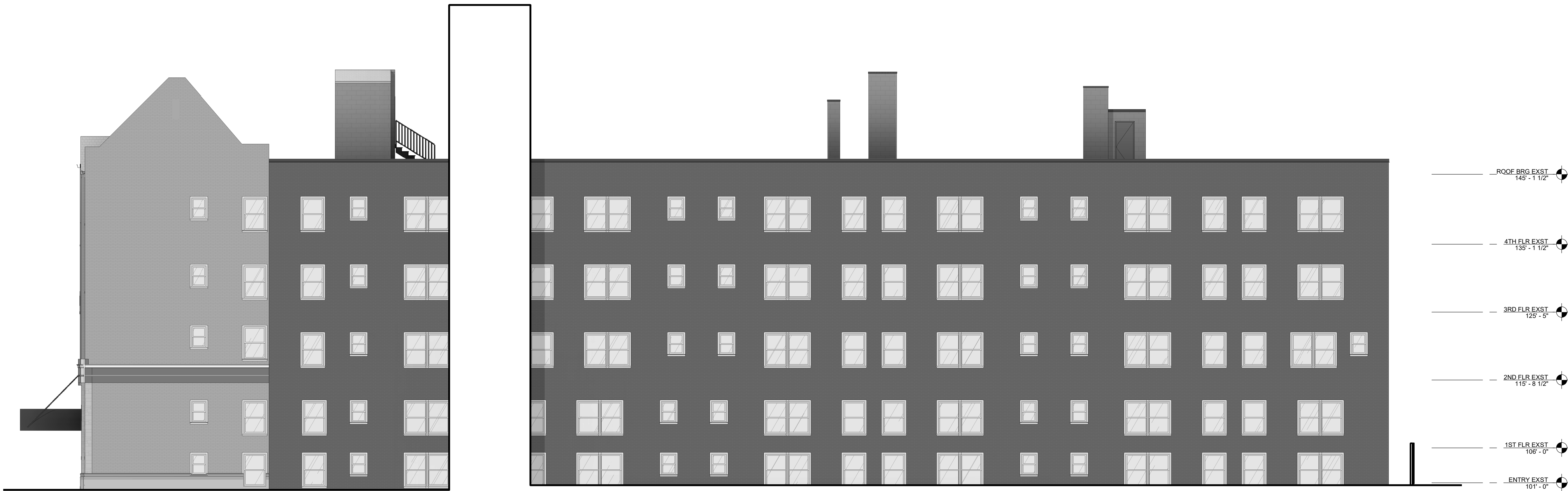
1 A4.2 WEST ELEVATION 1/8" = 1'-0"
