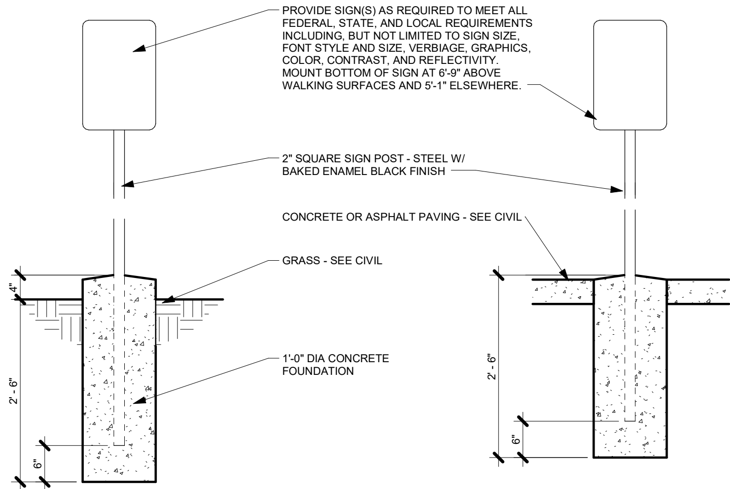
6 ACCESSIBLE PARKING SIGN DETAIL AS1.1 3/4" = 1'-0"
