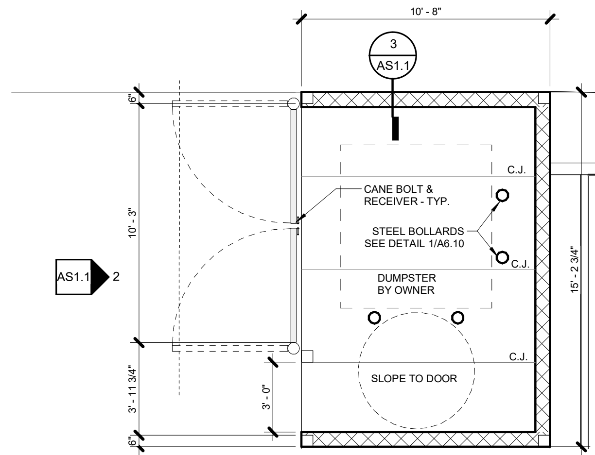
1 TRASH ENCLOSURE PLAN AS1.1 1/4" = 1'-0"
