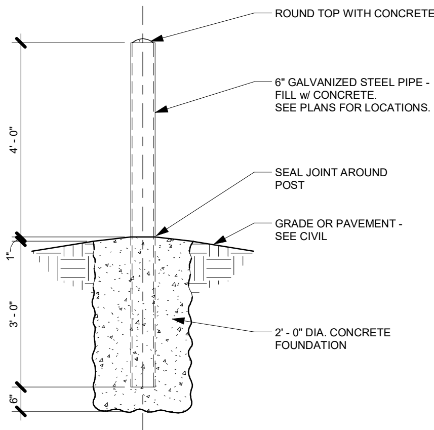
4 STEEL BOLLARD DETAIL AS1.1 1/2" = 1'-0"
