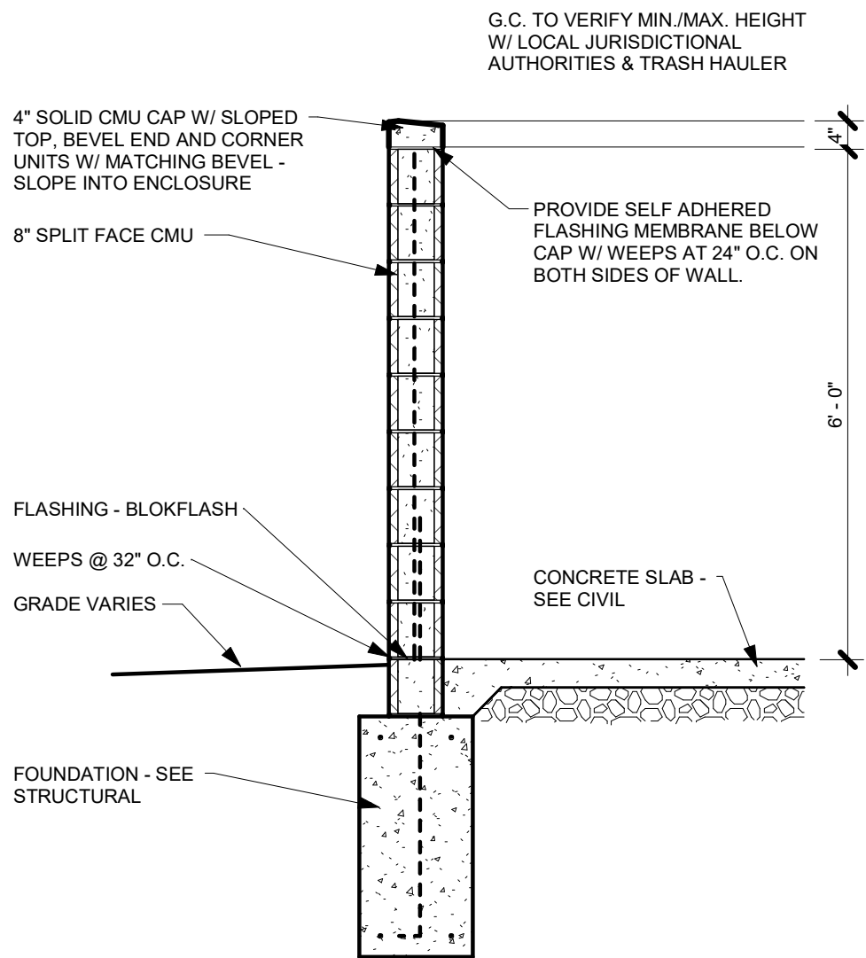
3 DUMPSTER WALL SECTION AS1.1 1/2" = 1'-0"
