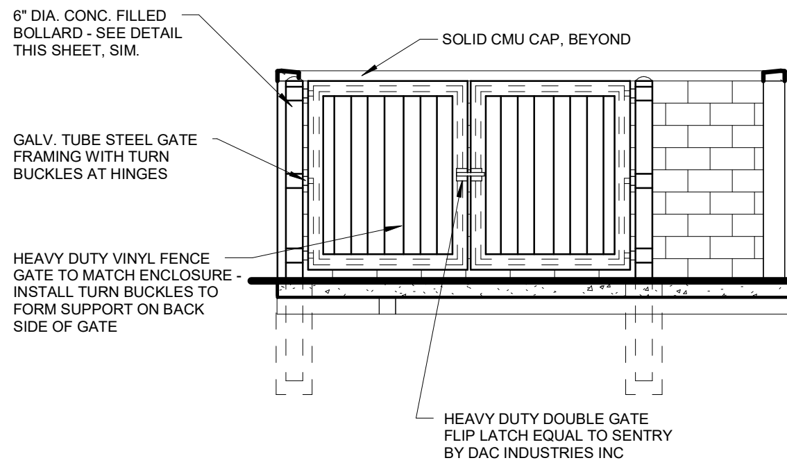
2 TRASH ENCLOSURE ELEVATION AS1.1 1/4" = 1'-0"
