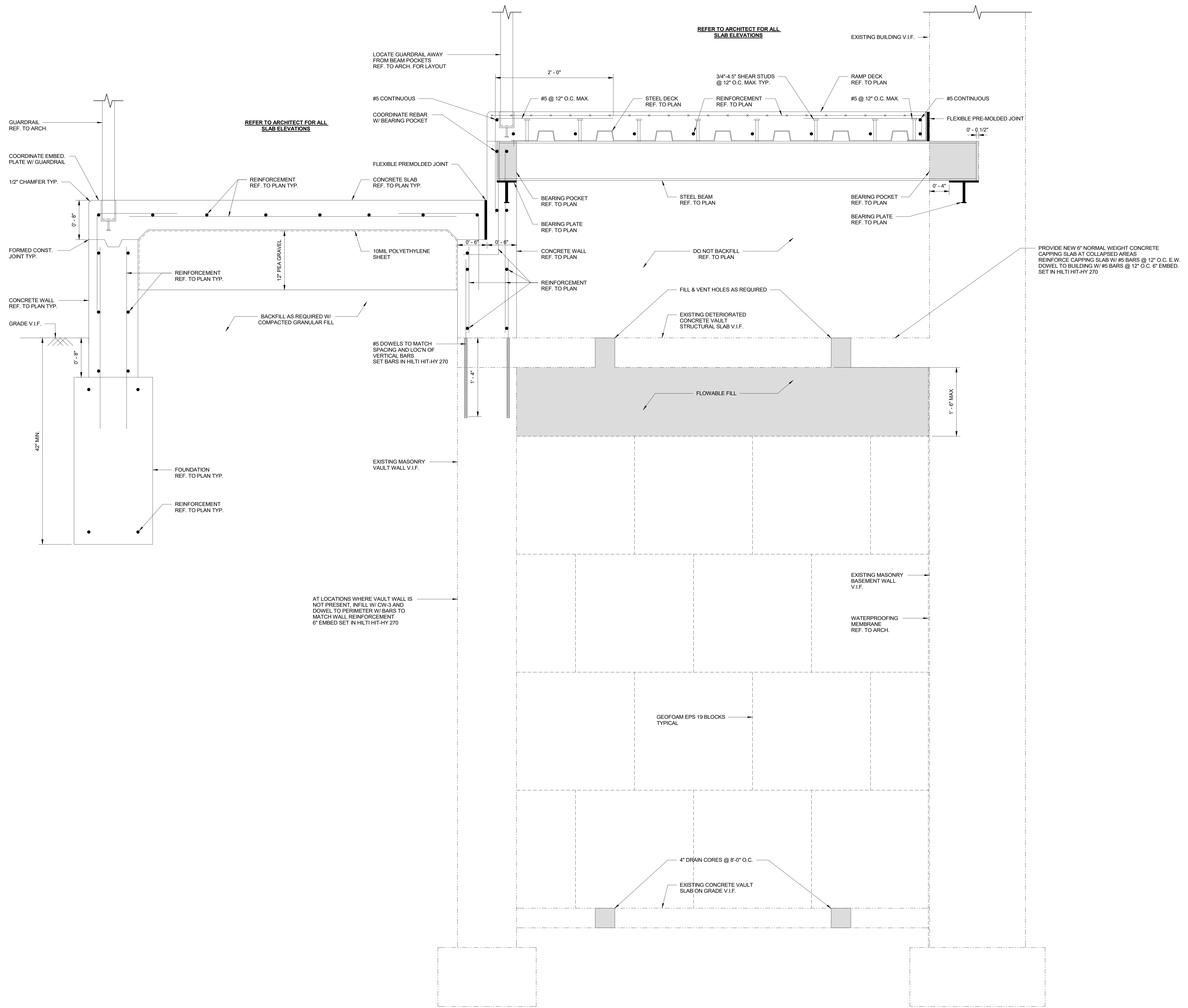
SECTION 2 1 1/2" = 1'-0"
