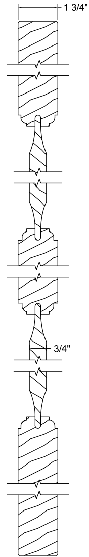
Section A-A 3/4" Single Hip Raised Panel
