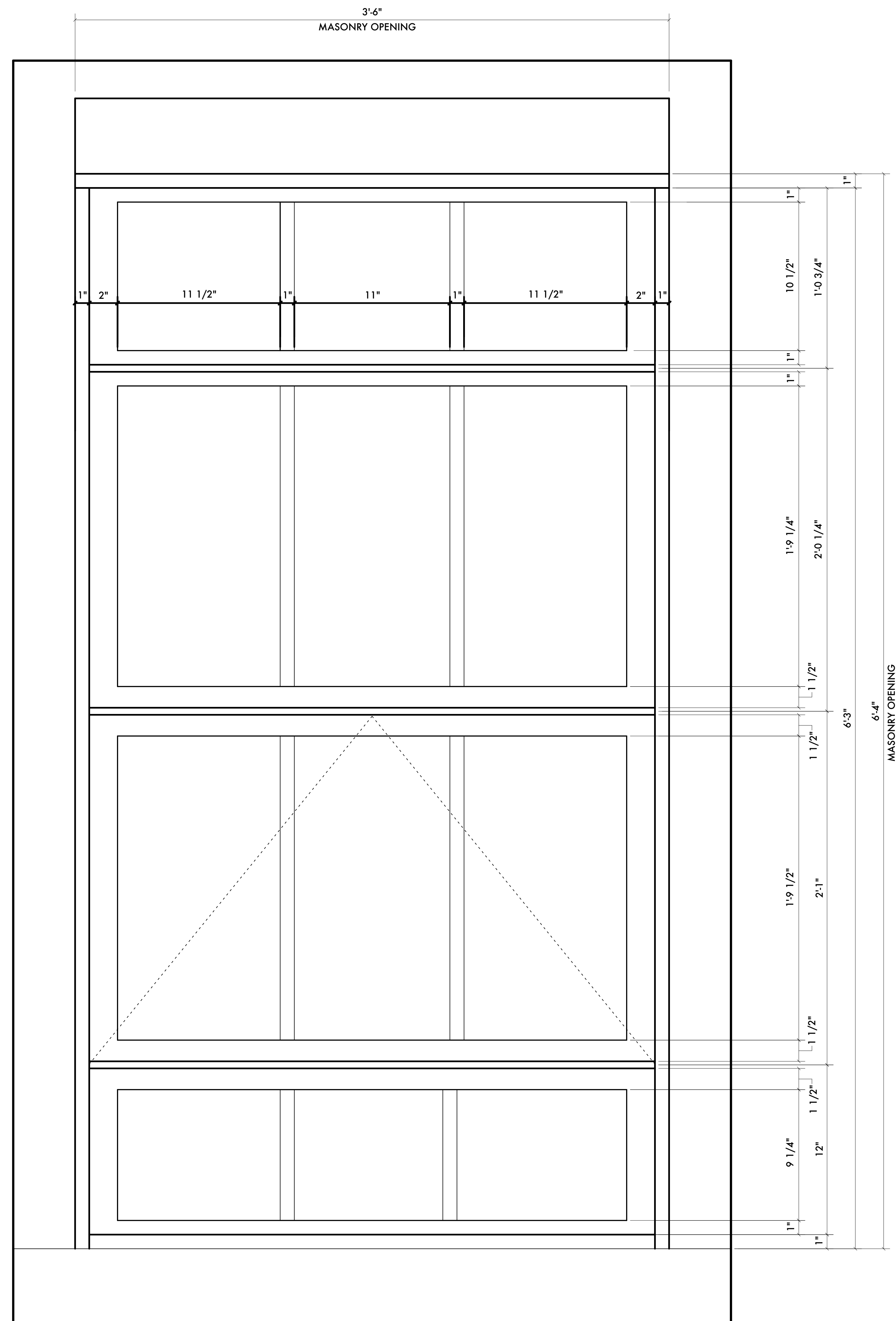
1 ENLARGED ELEVATION AT EXISTING WINDOW SCALE: 3" = 1'-0"
