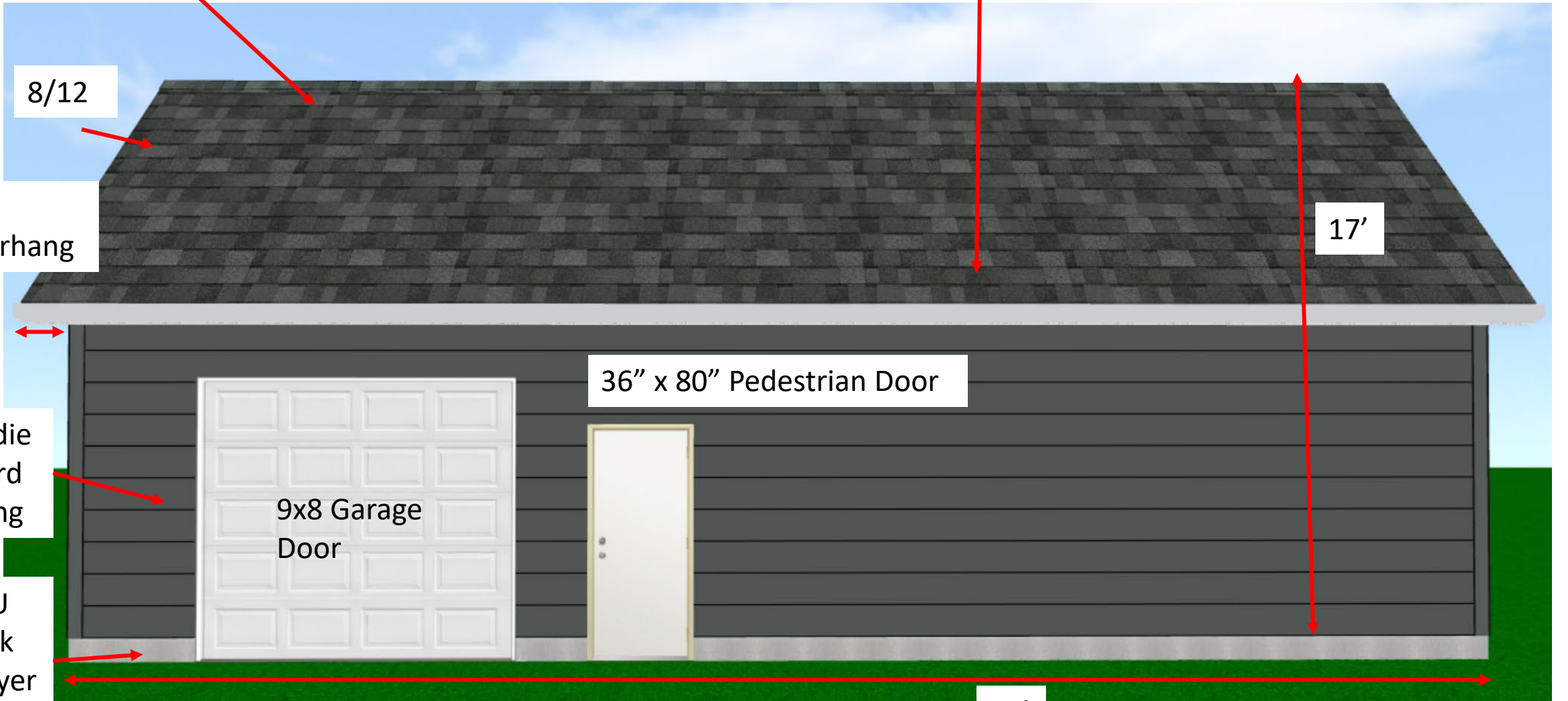
Elevation Plans – Yard Side
