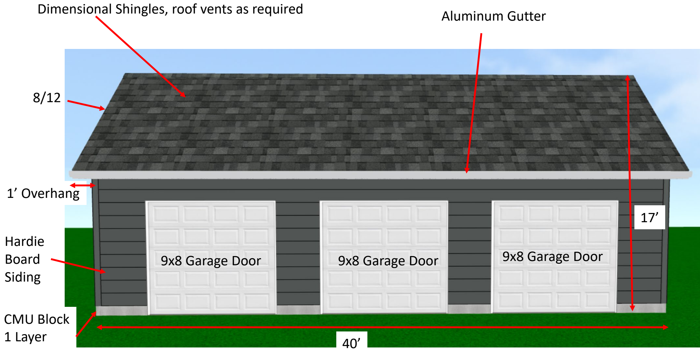
Elevation Plans – Alley Side
