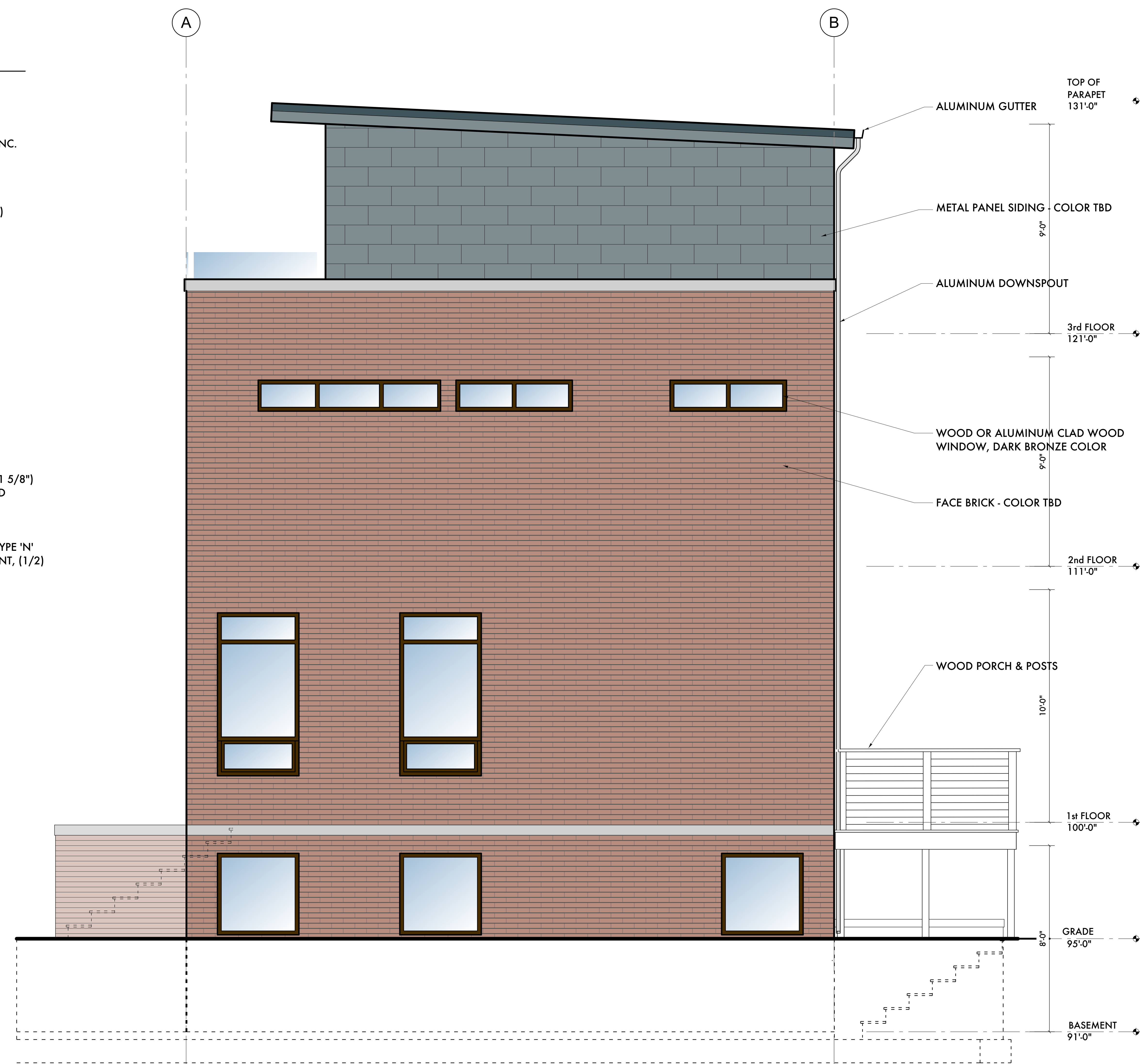
C SOUTH (LABROSSE) ELEVATION SCALE: 1/2" = 1'-0"
