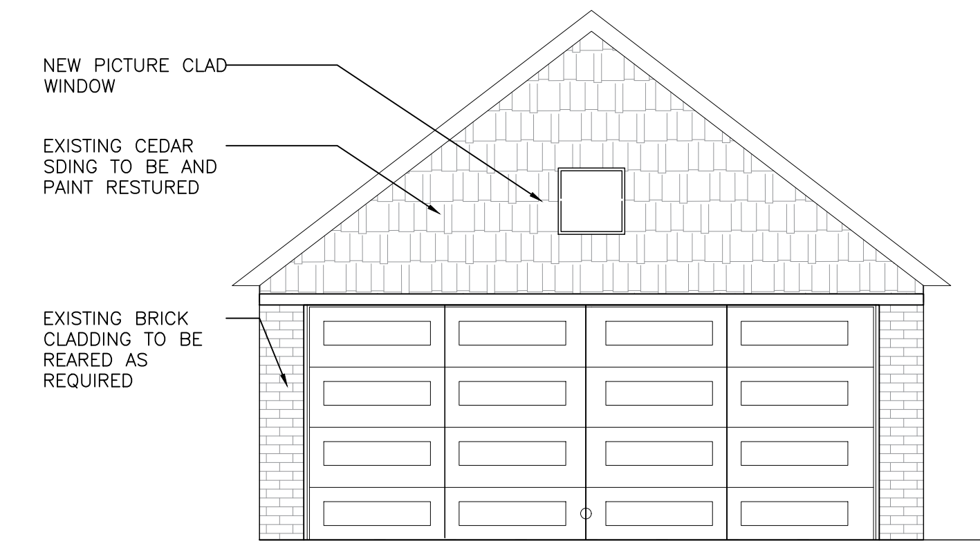
5 GARAGE ELEVATION VIEW A-200 SCALE: 1/4" = 1'-0"
