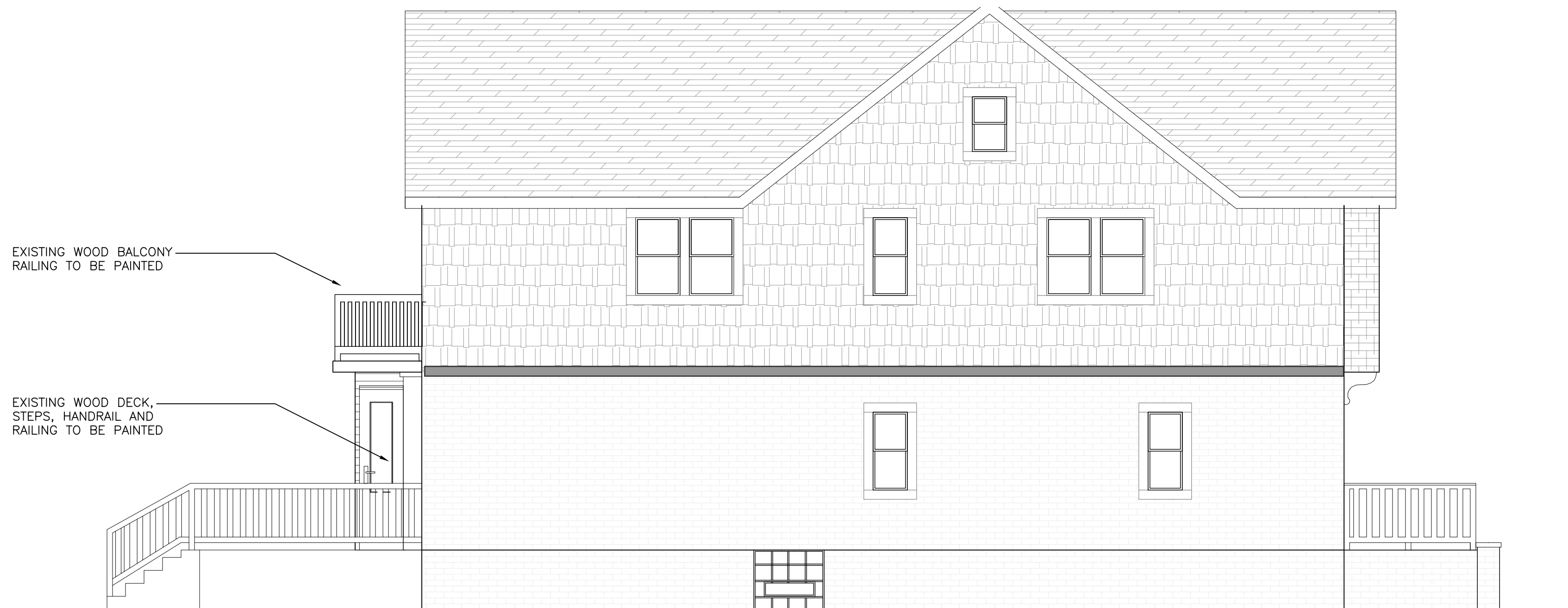
4 SOUTH ELEVATION VIEW A-200 SCALE: 1/4" = 1'-0"
