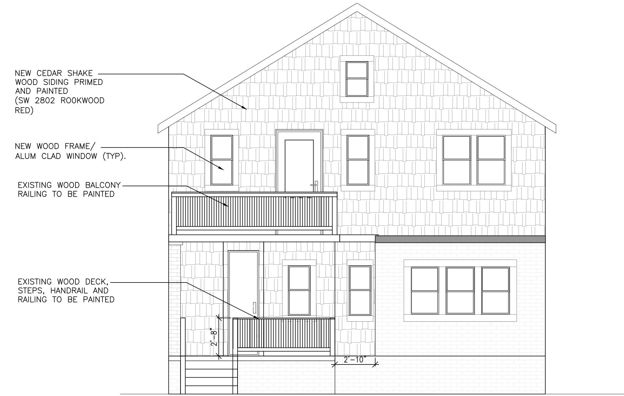
3 REAR ELEVATION VIEW A-200 SCALE: 1/4" = 1'-0"
