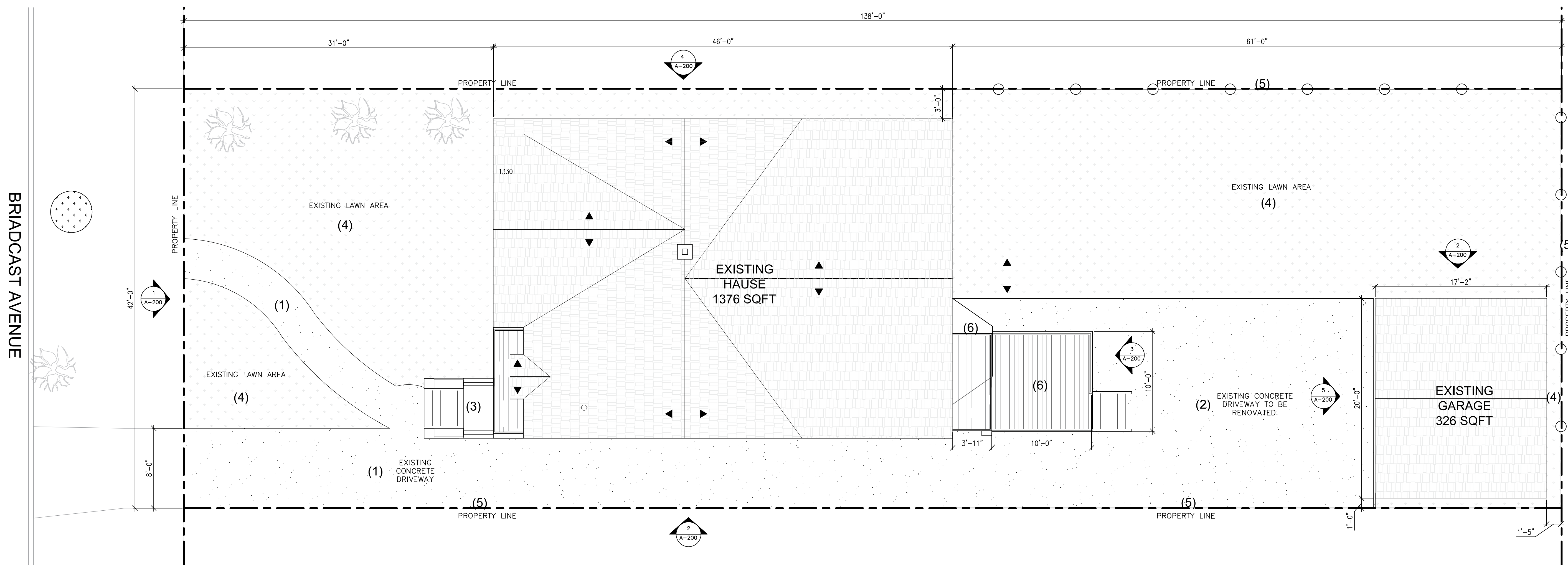
1 PROPOSAL SITE PLAN AS-101 SCALE: 3/16" = 1'-0"
