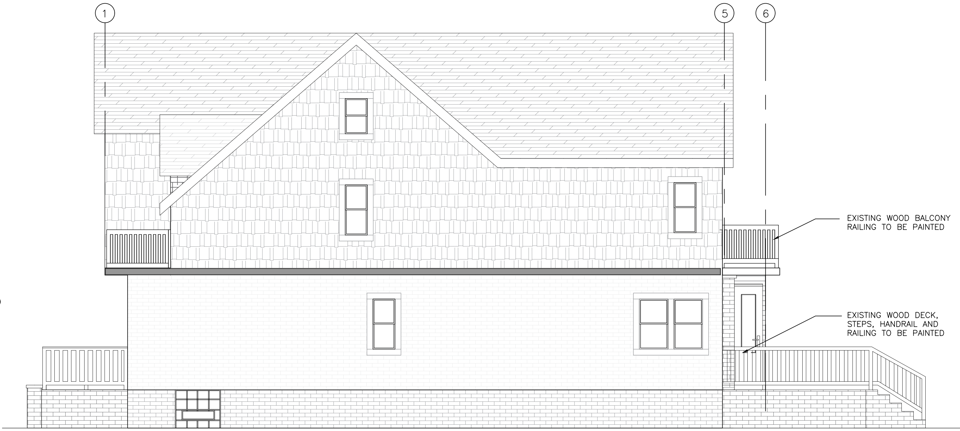
2 NORTH ELEVATION VIEW A-200 SCALE: 1/4" = 1'-0"
