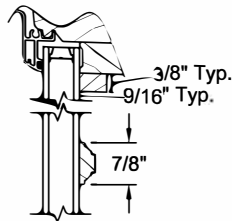
7/8" Full Surround
