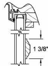
1 3/8" Full Surround
