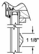
1 1/8" Full Surround
