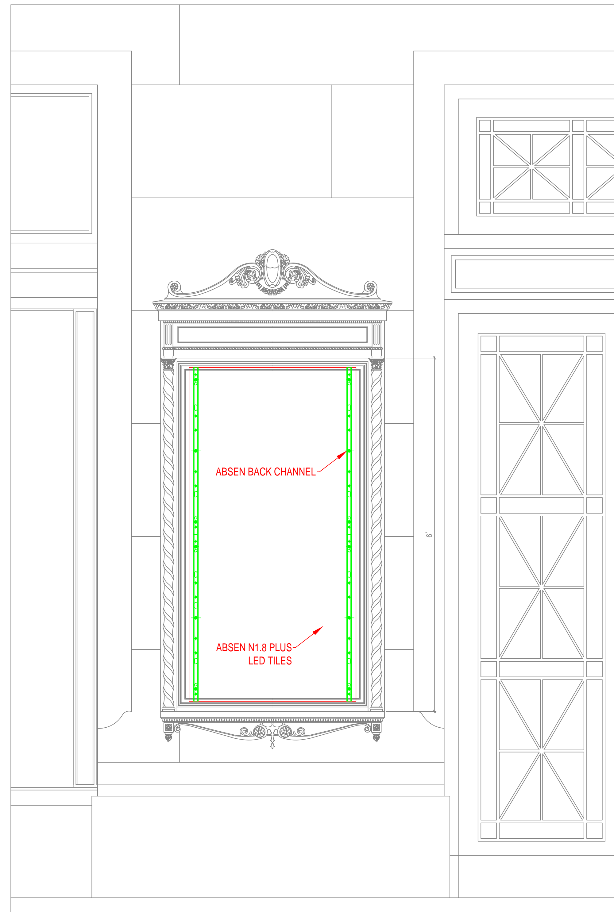
1 POSTER BOX ELEVATION 1" = 1'-0"
