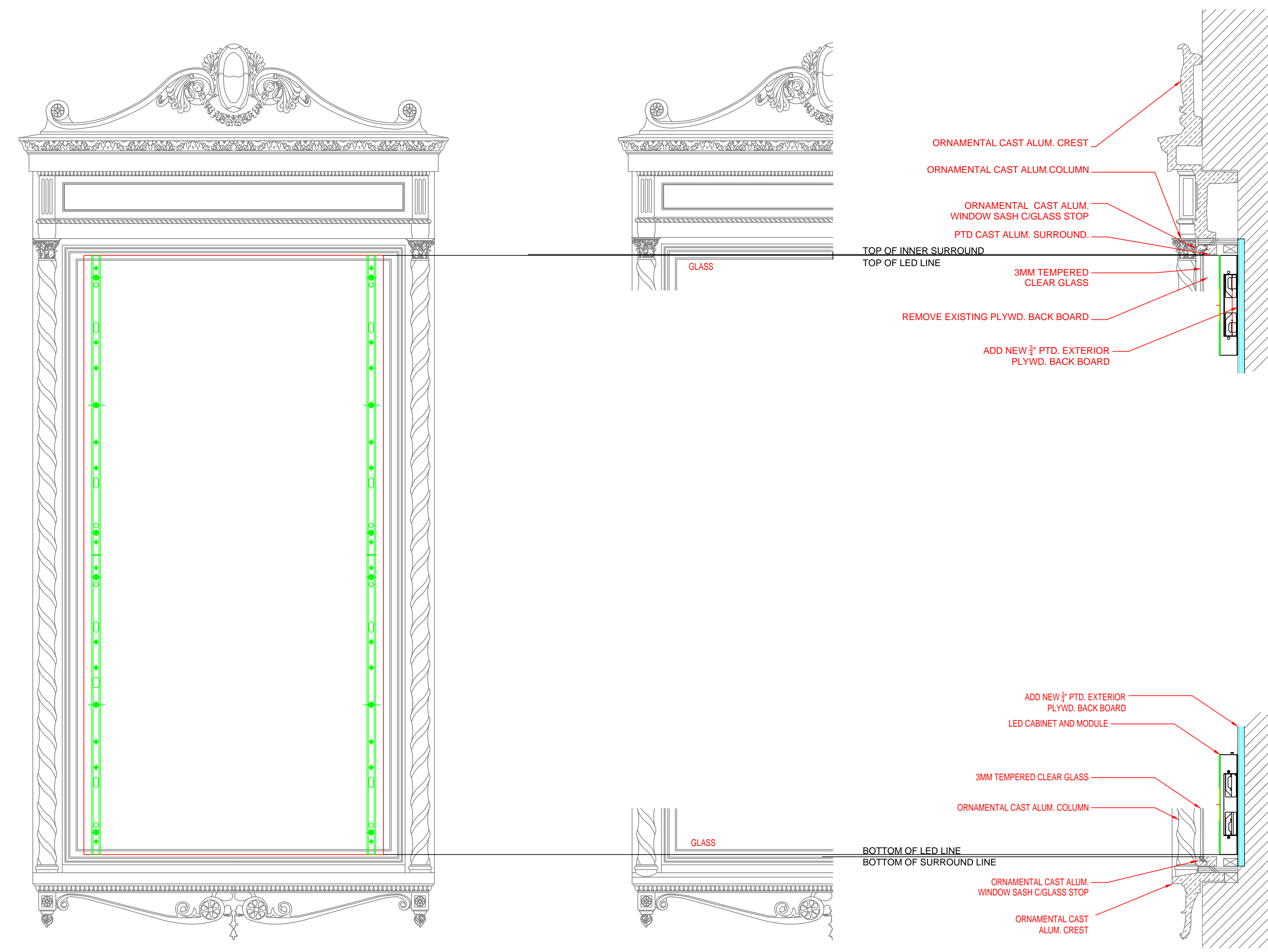
2 PART ELEV. PART PLAN POSTER BOX 1" = 1'-0"
