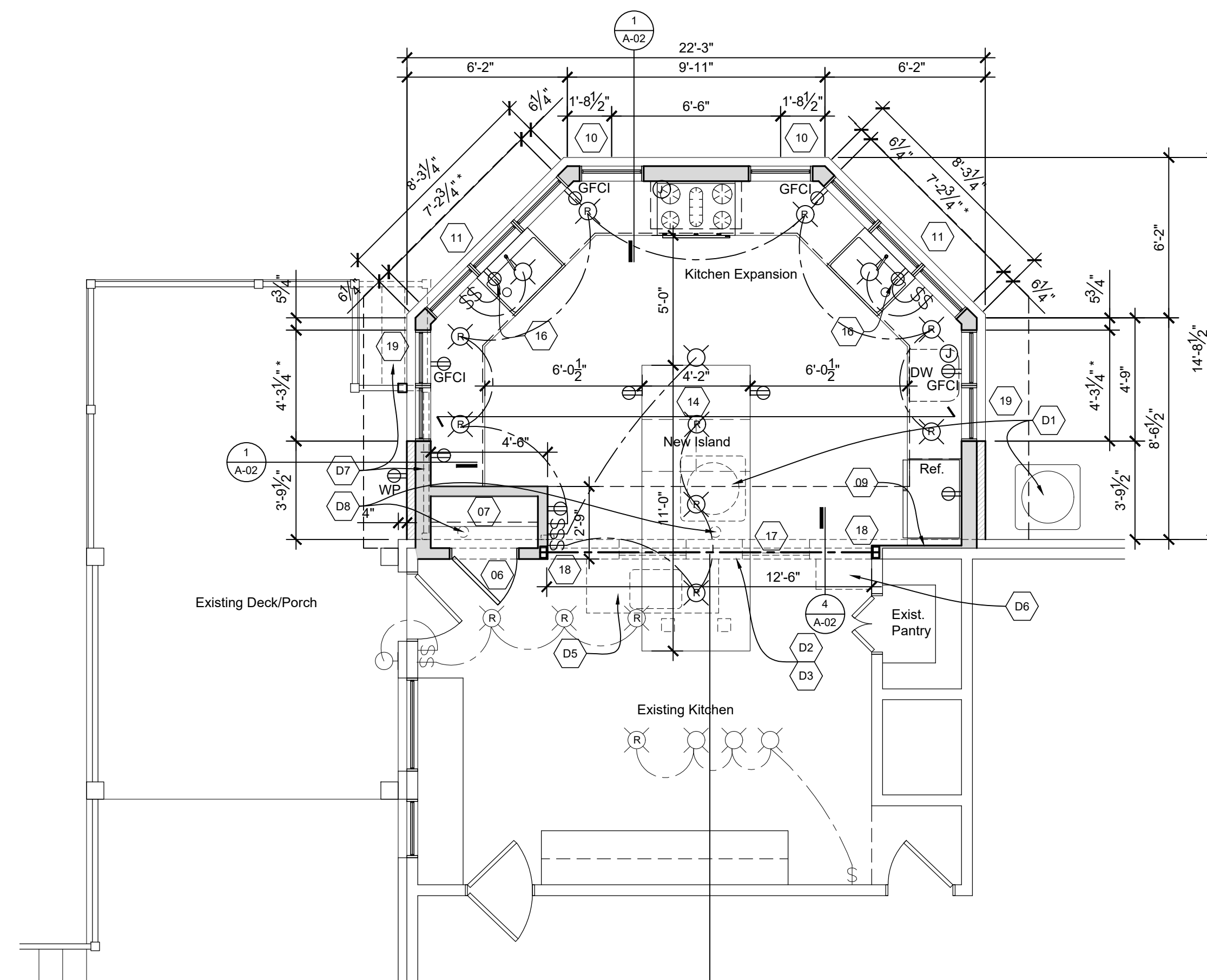
Floor Plan
