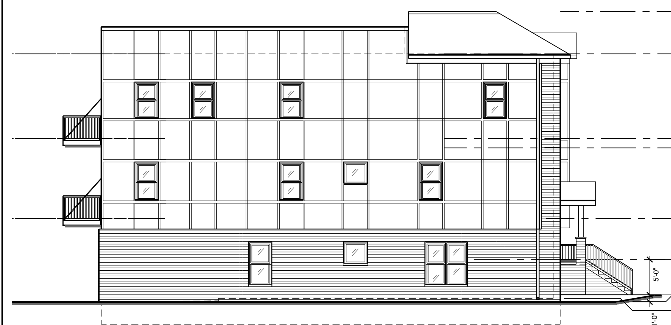
Side Building 2 - South Elevation Vehicle Drive SCALE: 1/8" = 1'-0" 4 - UNIT BUILDING
