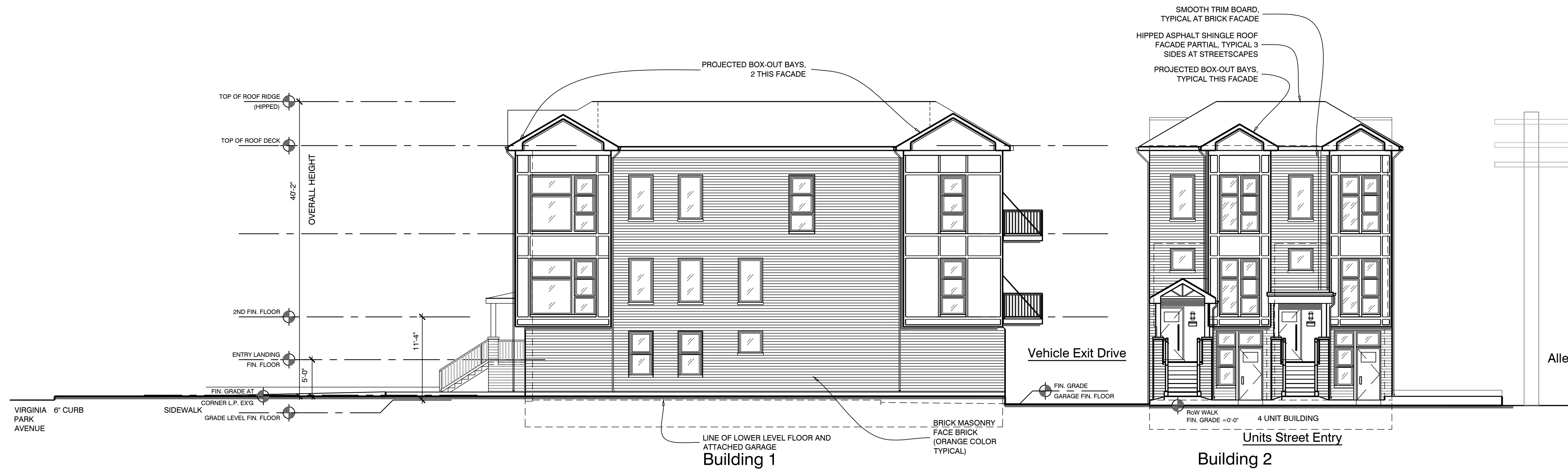
Side - East Elevation
