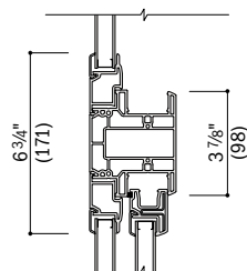
Vertical Section Picture Over Gliding
