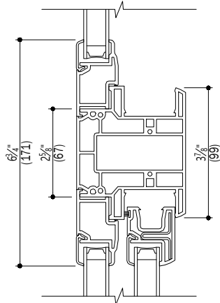
B 3 Horizontal Integral Join Stationary/Operating Stationary Side
