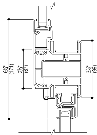
A 3 Horizontal Integral Join Stationary /Operating
