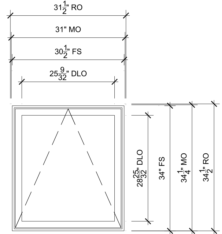
KITCHEN SCALE: 3/4" = 1'-0" Head, Sill, Jamb, Check Rail
