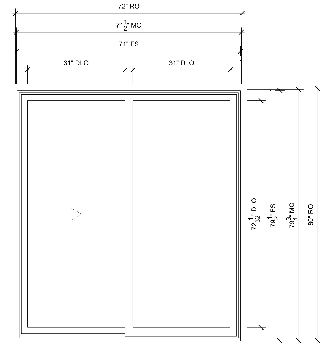
BREAKFAST NOOK SCALE: 3/4" = 1'-0" Head, Meeting Stile, Jamb, Jamb, Sill
