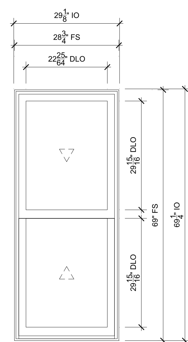
BAR SCALE: 3/4" = 1'-0" Head, Sill, Jamb, Check Rail
