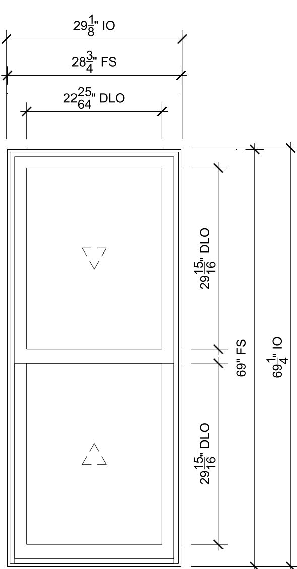
BEDROOM 1 SCALE: 3/4" = 1'-0" Head, Sill, Jamb, Check Rail
