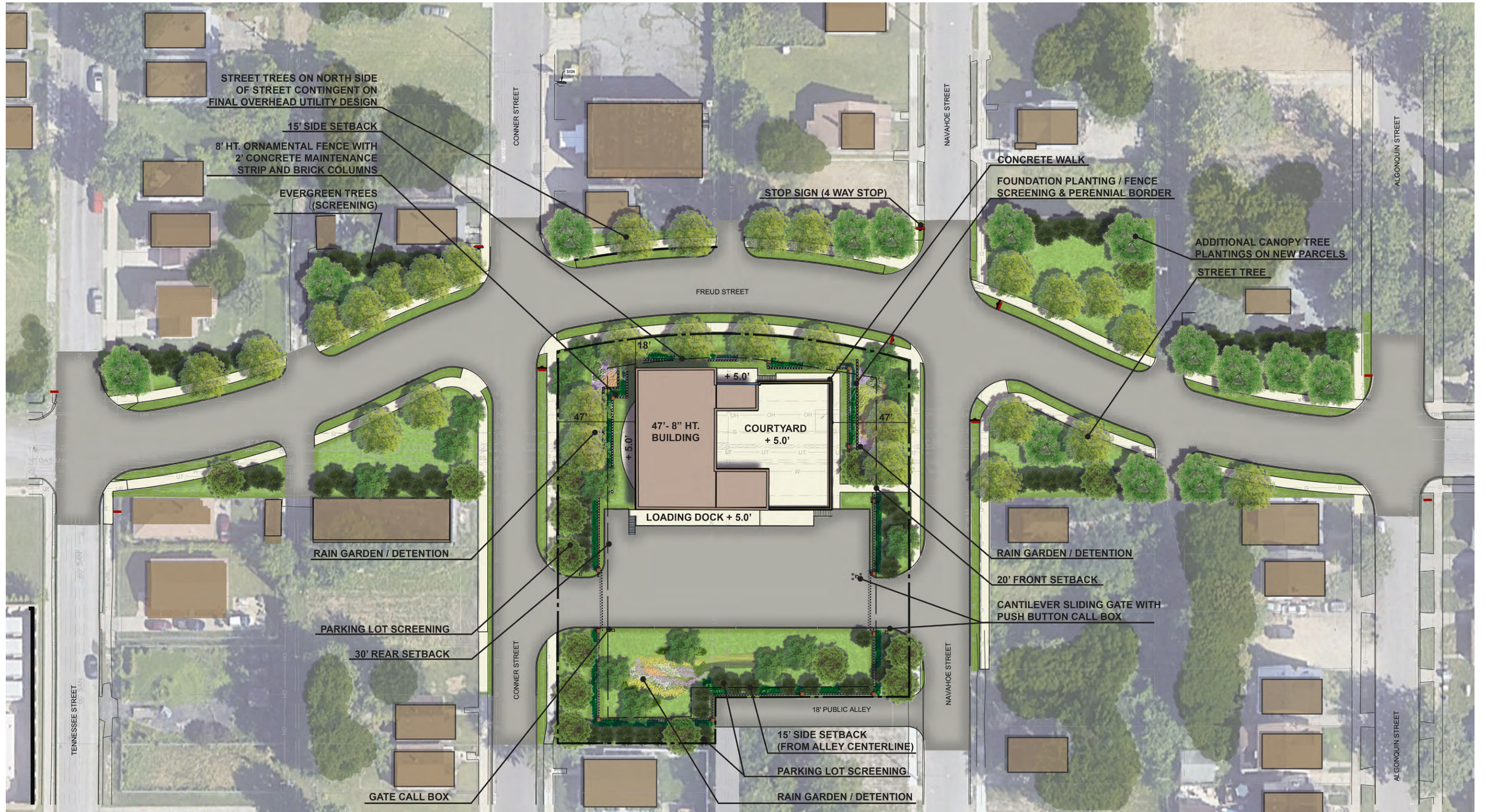
Freud Sanitary Pump Station Site Plan
