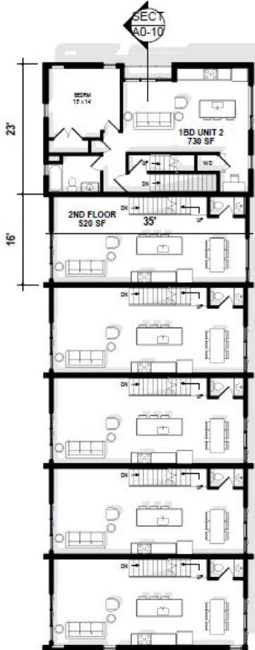
2 PROPOSED 2ND FLOOR PLAN 1/16" = 1'-0"
