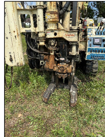
Photo 4: Viewing 14425 SB02 Drilling, Facing North.
