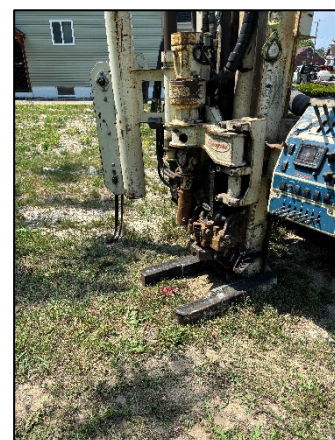
Photo 6: Viewing 14160 SB03 Drilling, Facing West.
