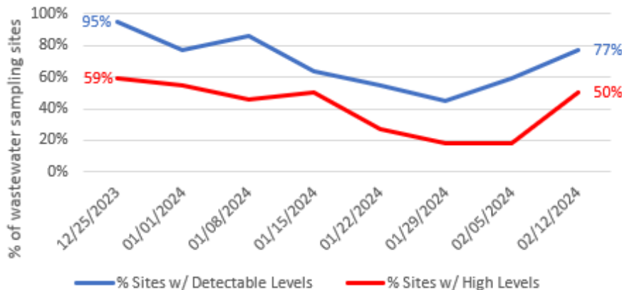
Figure 4: SARS-CoV-2 Wastewater Levels
