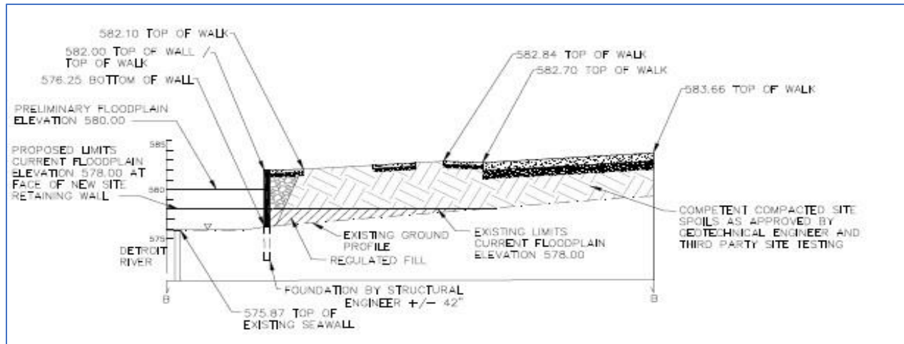
Figure 2- Floodplain Impact Cross Section
