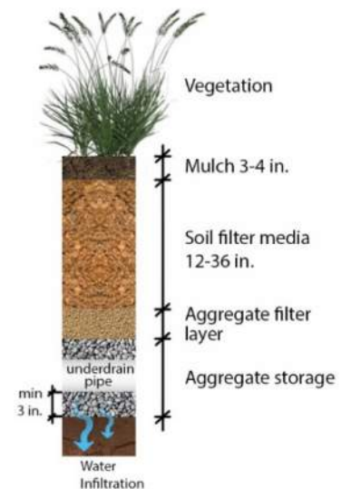
Figure 8-12 Typical Conventional profile
