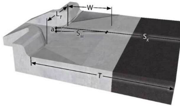
Figure 5-6 Depressed Curb Opening Cross Section
