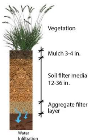
Figure 8-14 Typical Pipeless profile
