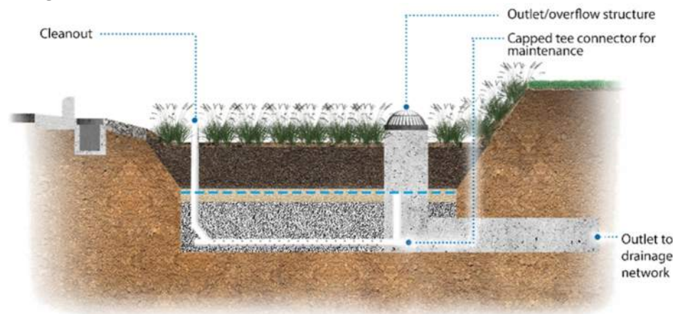
Figure 8-28 Bioretention cell with a saturated zone drainage profile
