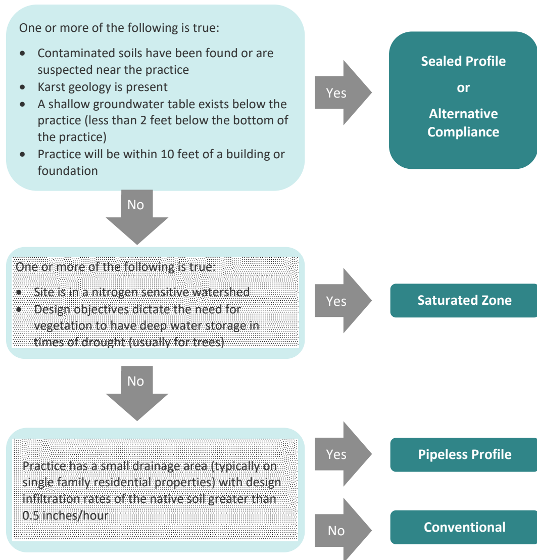
Figure 8-16 Drainage profile selection
