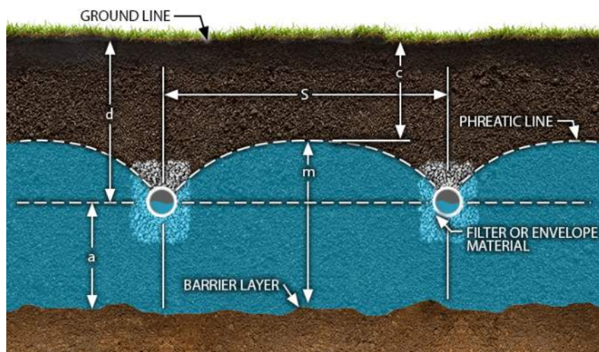
Figure 5-11 Ellipse Equation Variables
