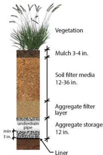
Figure 8-15 Typical sealed profile
