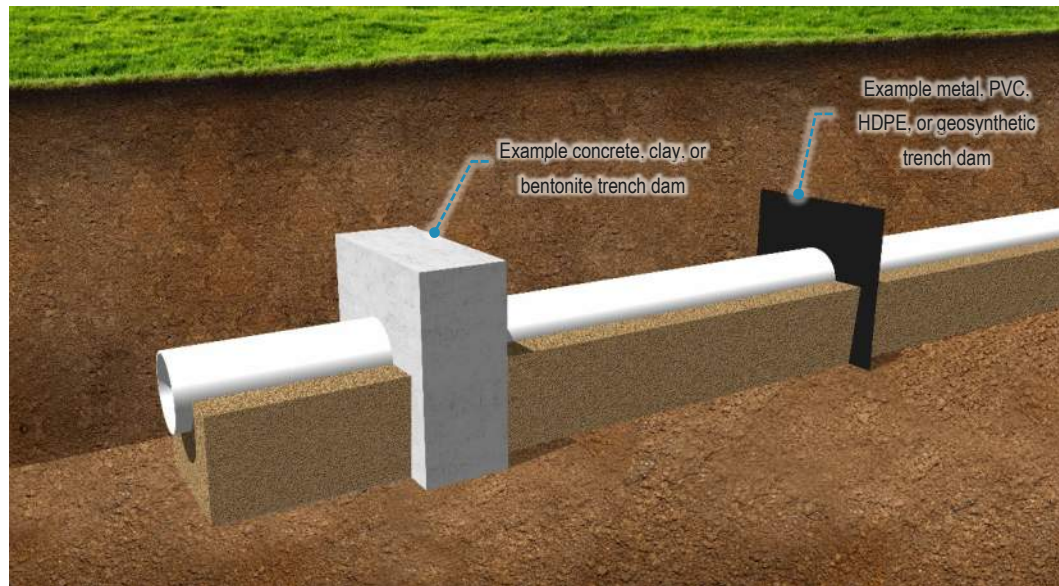
Figure 5-10 Trench dam
