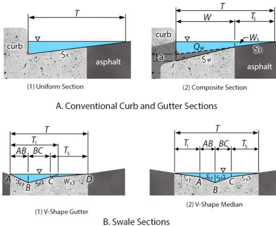
Figure 5-2 Typical Curb and Gutter Sections
