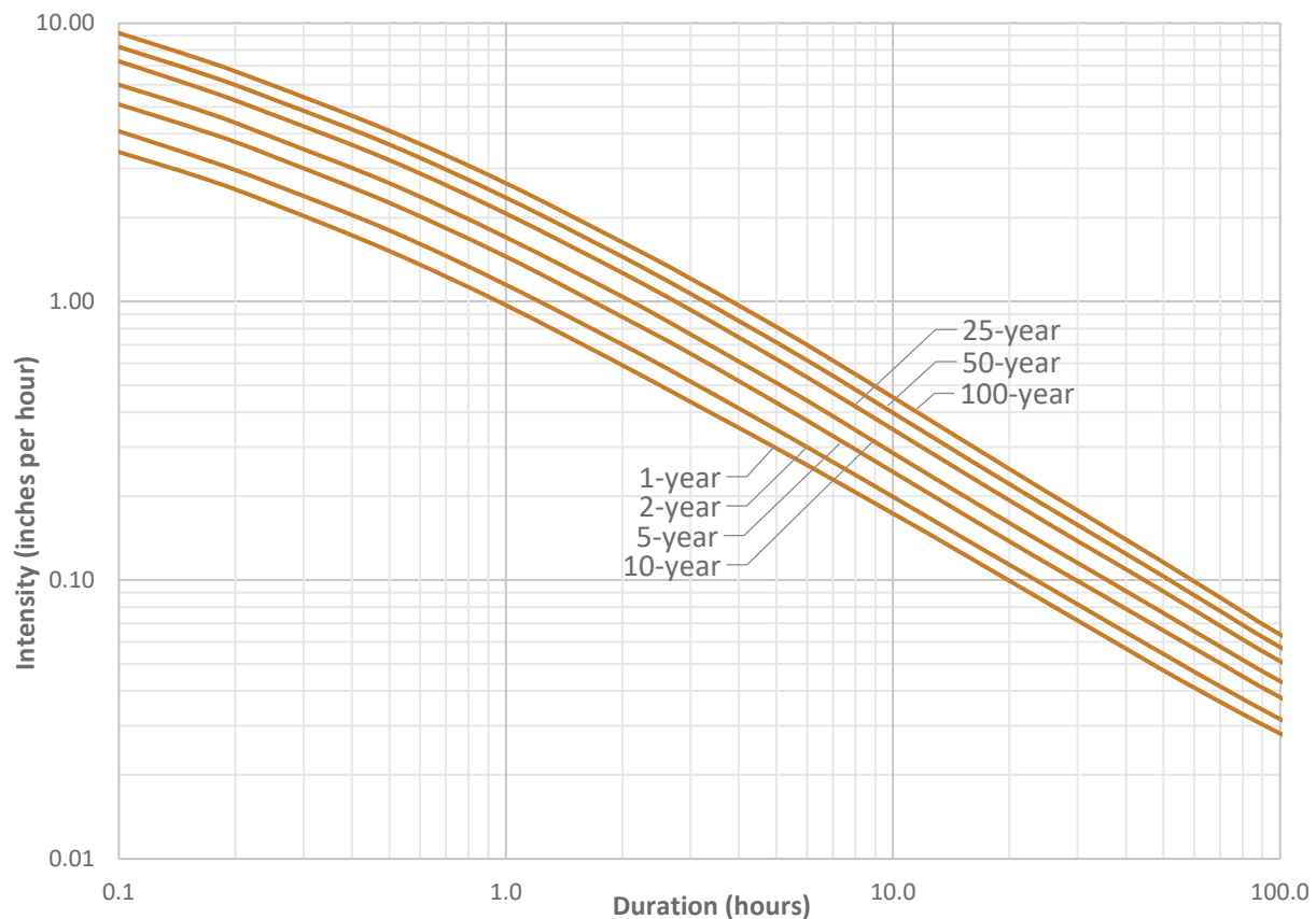
Figure 4-1 Intensity Duration Frequency (IDF) Curves for Detroit based on NOAA Atlas 14 Data
