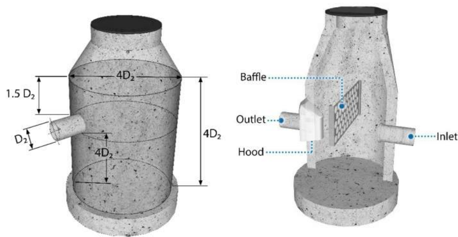
Figure 5-8 Inlet Structure with Sediment Sump
