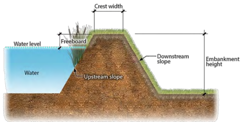
Figure 7-7 Embankment Illustration
