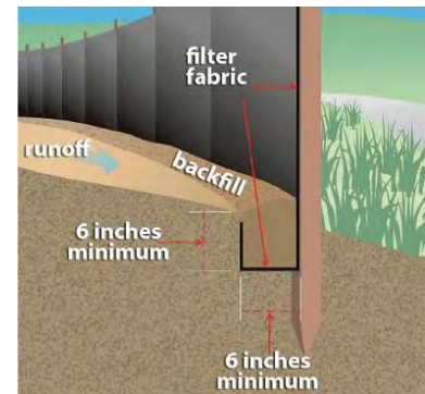
Figure 3-14 Silt fence
