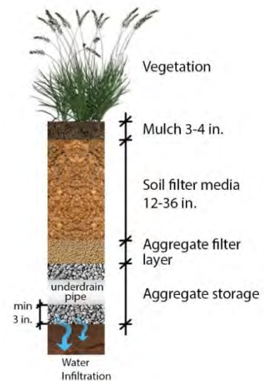
Figure 8-12 Typical conventional drainage profile
