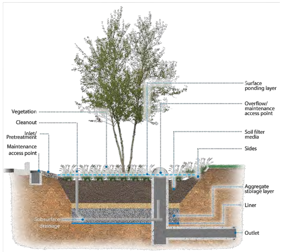
Figure 8-1 Components of a typical bioretention practice
