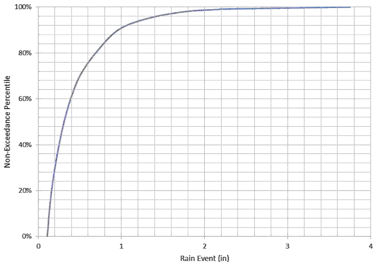
Figure 4-2 Non-Exceedance Rainfall
