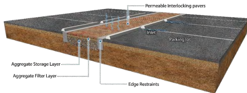
Figure 10-1 Permeable interlocking concrete pavers in a parking lot
