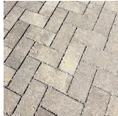
Figure 10-5 Example of Permeable Interlocking Concrete Pavers
