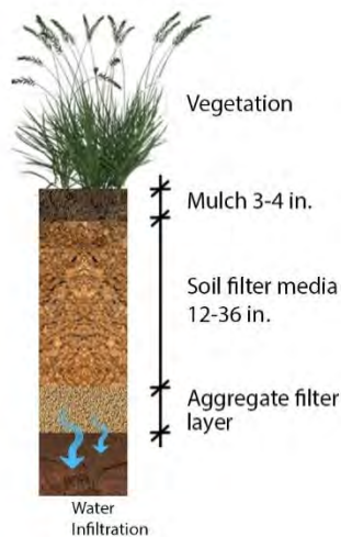
Figure 8-14 Typical pipeless practice profile
