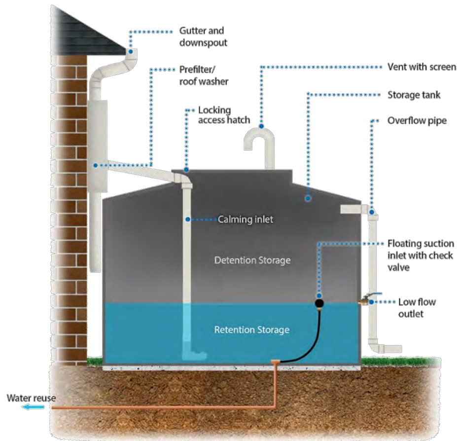
Figure 11-8 Cistern for detention and retention storage
