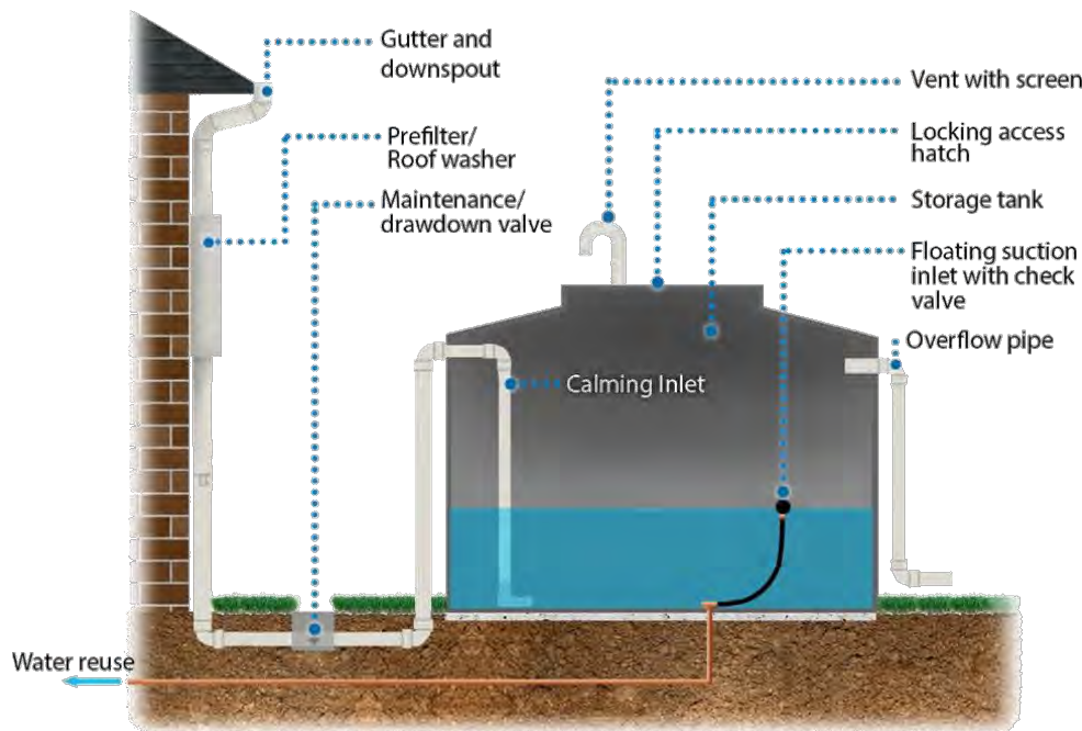
Figure 11-4 Cistern with wet conveyance featuring a drawdown valve for maintenance
