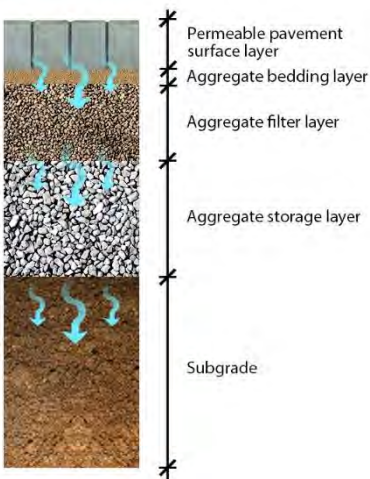
Figure 10-18 Typical pipeless drainage profile
