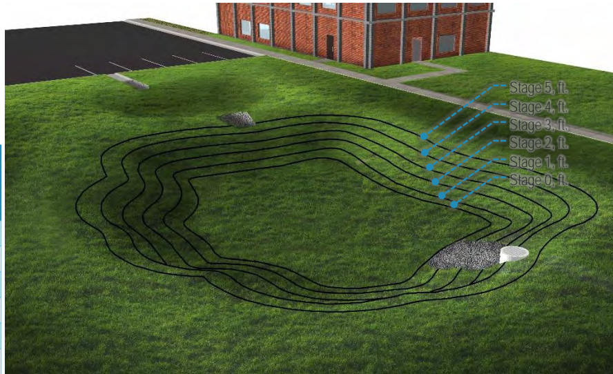
Figure 7-13 Example Detention Basin
