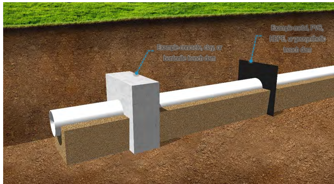
Figure 5-10 Trench dam
