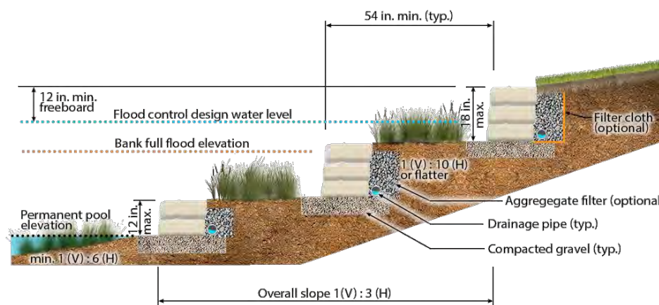
Figure 13-8 Terraced Side Slopes
