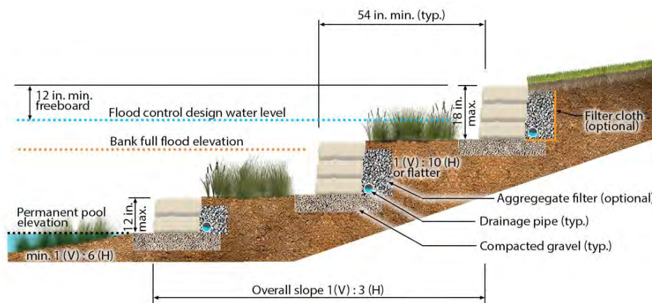
Figure 9-14 Terraced side slopes on an infiltration basin
