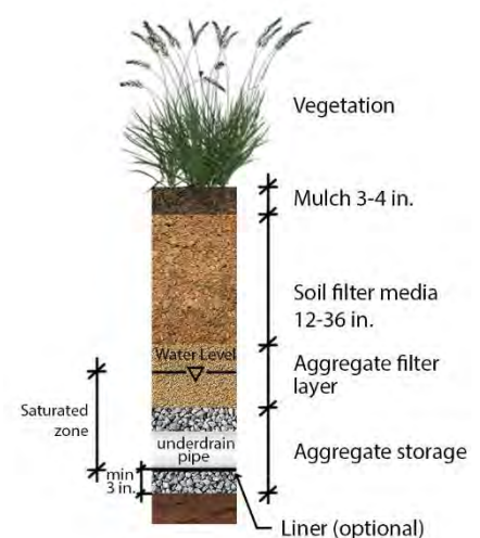
Figure 8-13 Typical saturated zone profile
