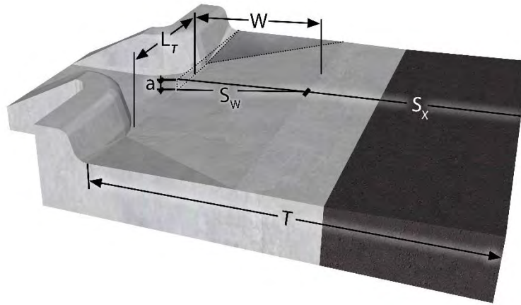
Figure 5-6 Depressed Curb Opening Cross Section
