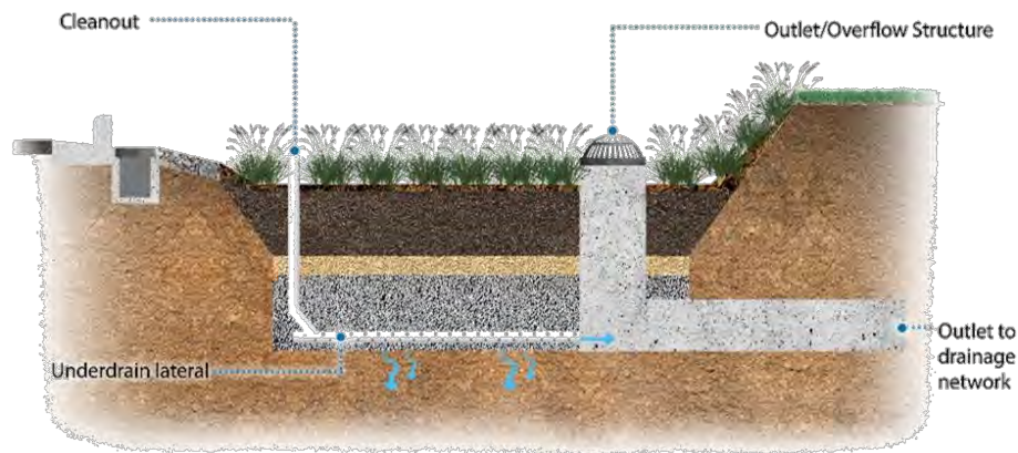
Figure 8-27 Bioretention cell with a conventional drainage profile
