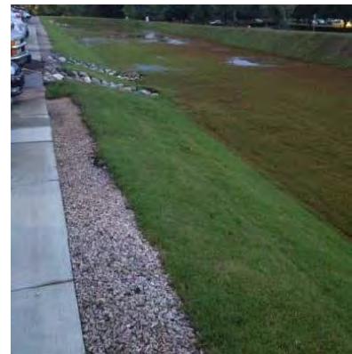
Figure 8-21 Gravel fringe flow spreader
