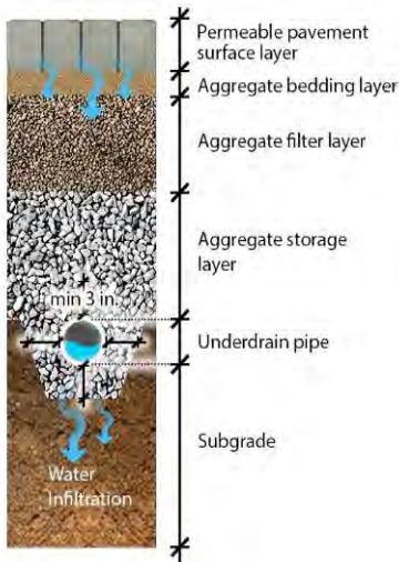
Figure 10-17 Typical conventional drainage profile
