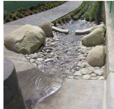
Figure 8-25 Armored inlet
