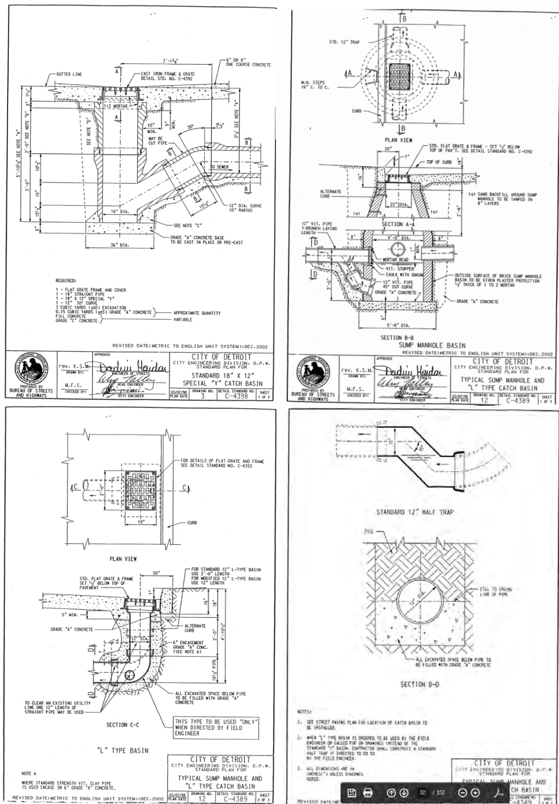
Figure 5-7 Standard Inlet Structures
