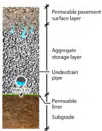
Figure 10-24 Single depth aggregate storage layer
