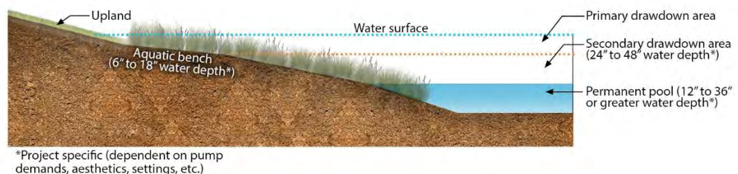
Figure 7-12 Hydraulic Profile of Detention Practice for Reuse
