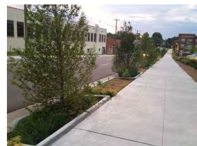
Figure 8-17 Vertical curbing adjacent to sidewalk
