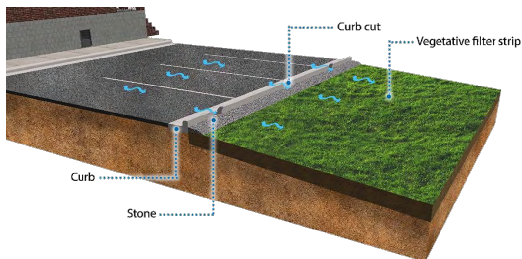
Figure 5-13 Typical Level Spreader
