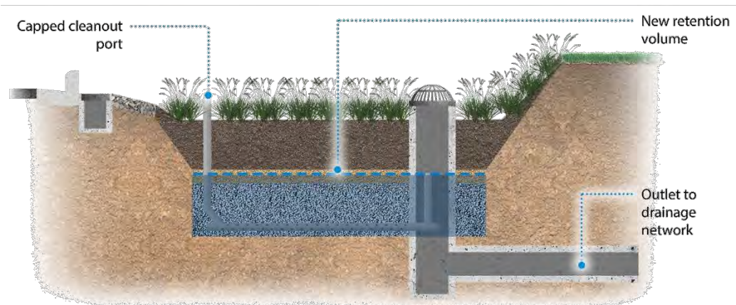
Figure 8-31 Cross sectional area of volume retained with an underdrain
