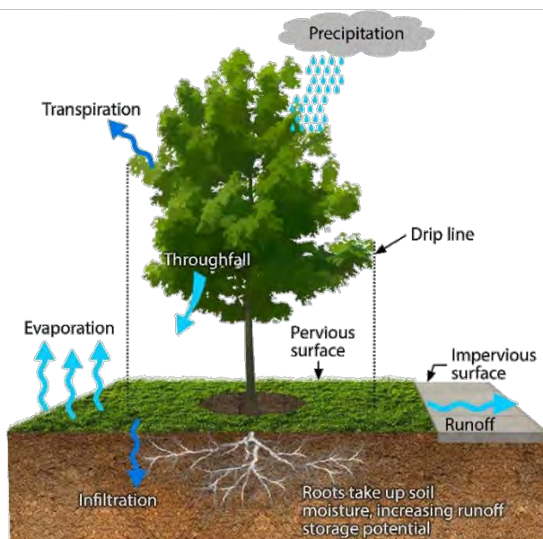
Figure 15-1 The role of trees in the hydrologic cycle
