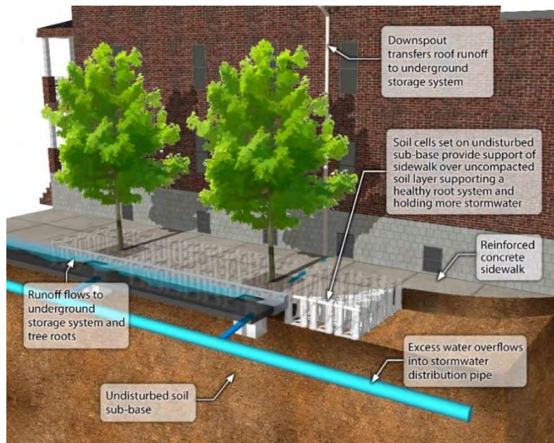
Figure 15-4 Typical suspended pavement system
