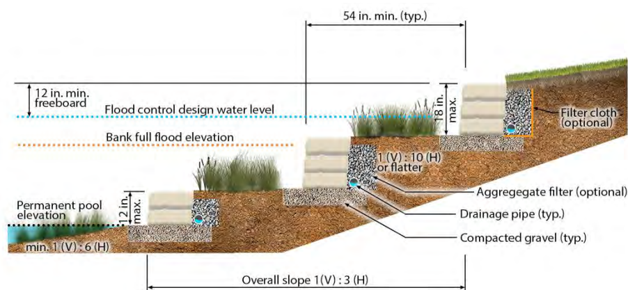
Figure 7-8 Terraced Side Slopes
