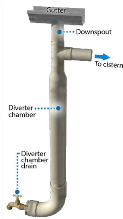
Figure 11-6 First-Flush Diverter
