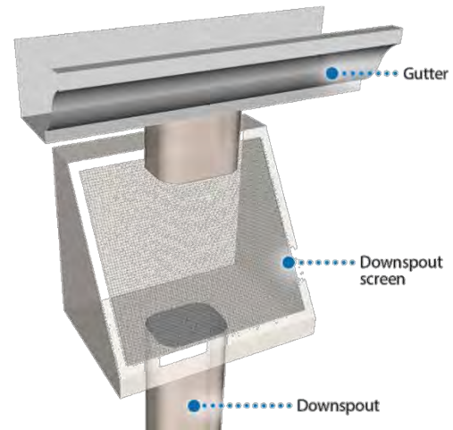
Figure 11-5 Debris Excluder
