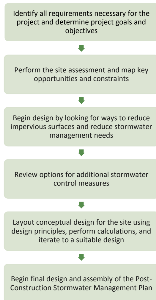
Figure 3-1 Integrated Site Design Process
