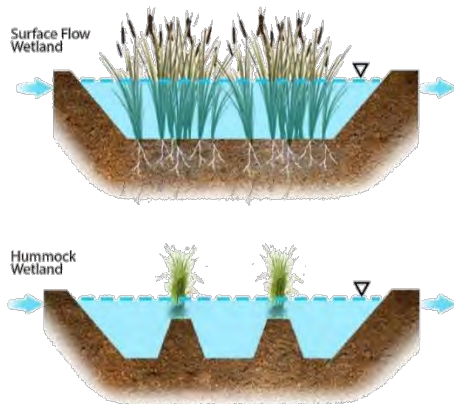
Figure 13-4 Wetland Variants
