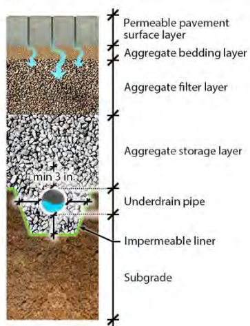
Figure 10-28 Sealed Drainage Profile
