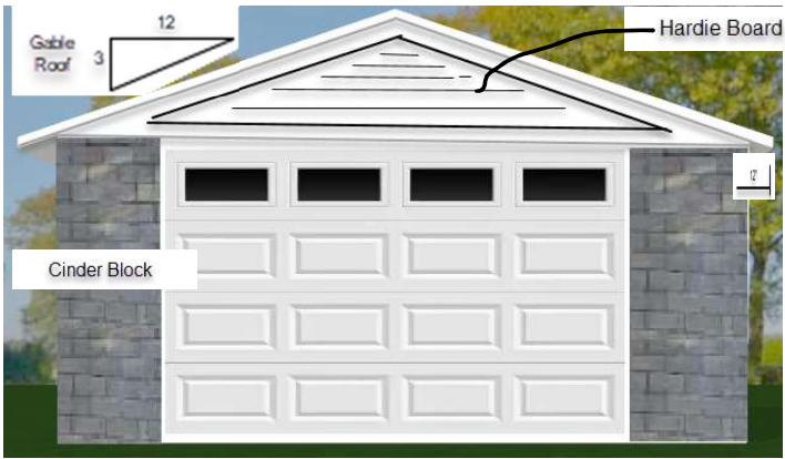
Front Garage Elevation
